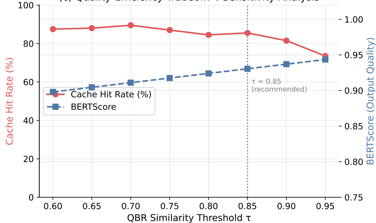
(c) Quality-Efficiency Tradeoff: \tau Sensitivity Analysis
