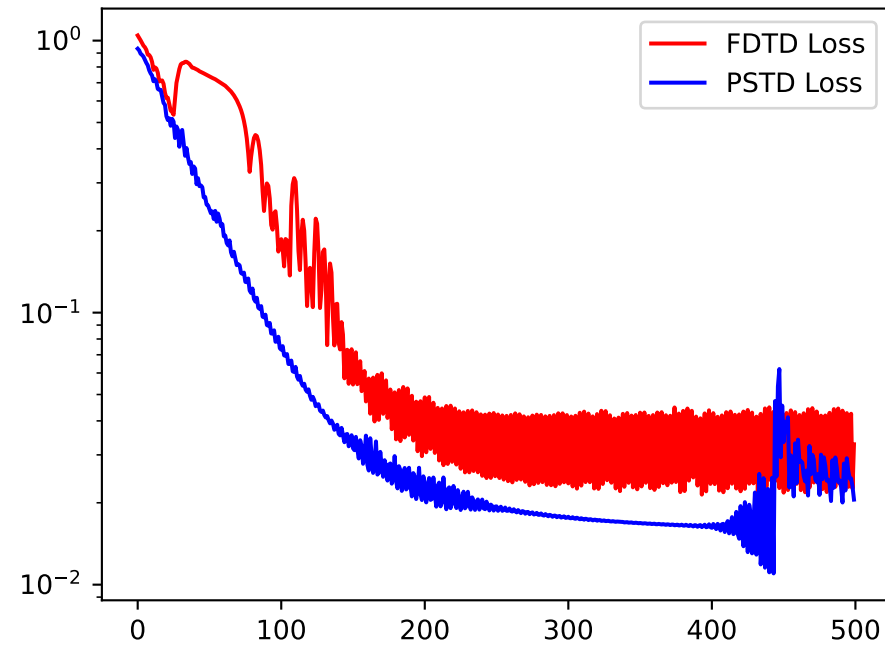
Training Loss
