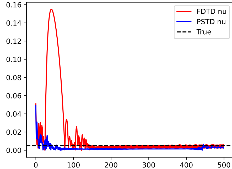
Nu Convergence
