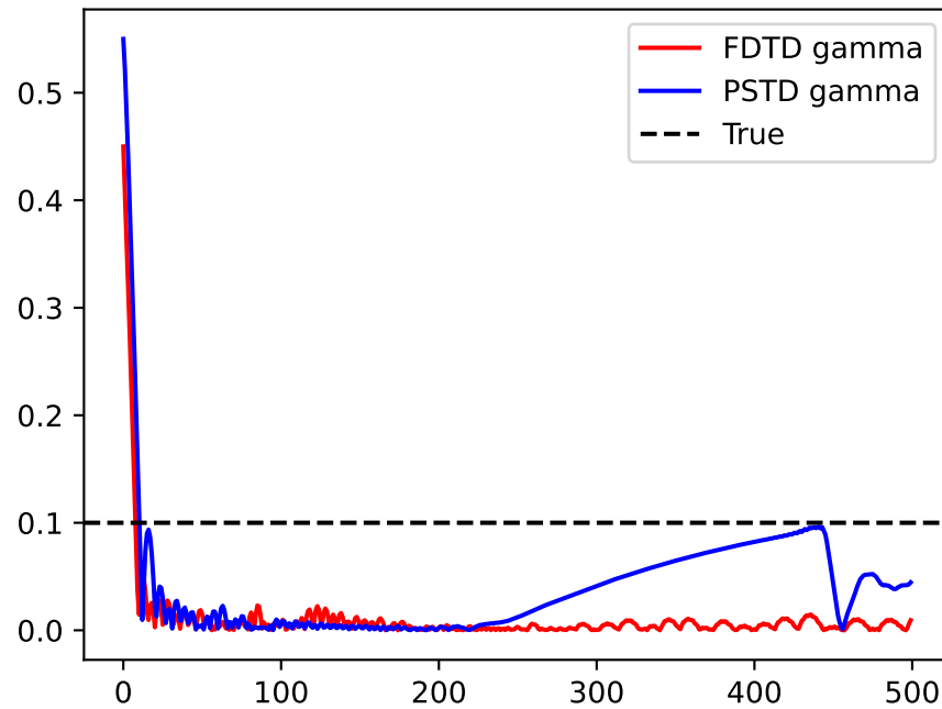
Gamma Convergence
