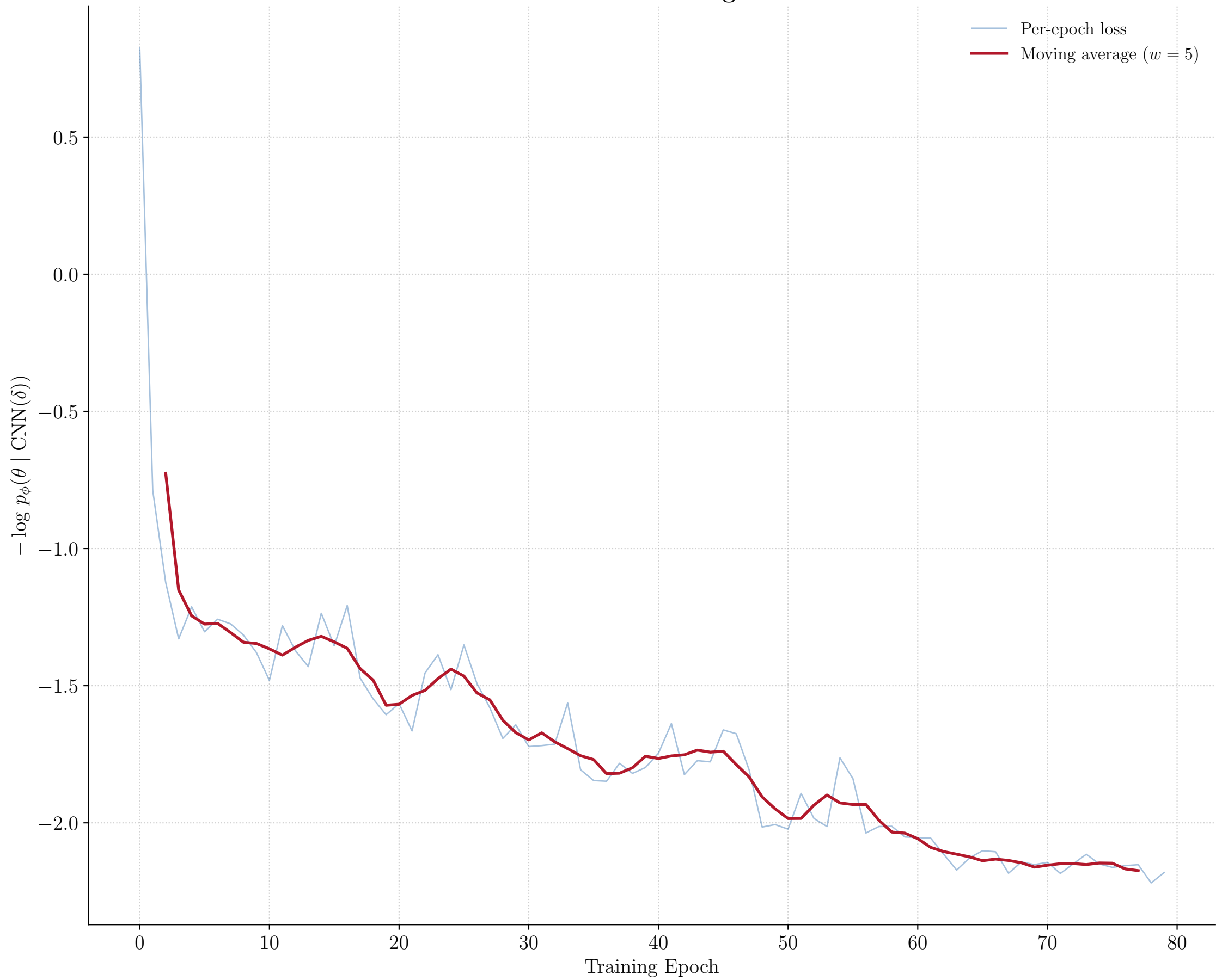
Field-NPE Training Loss
