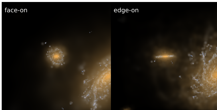
Subhalo 141036 [S] \log M_* = 10.74 DoR = 0.60 \log \Sigma_{1.5} = 10.47
