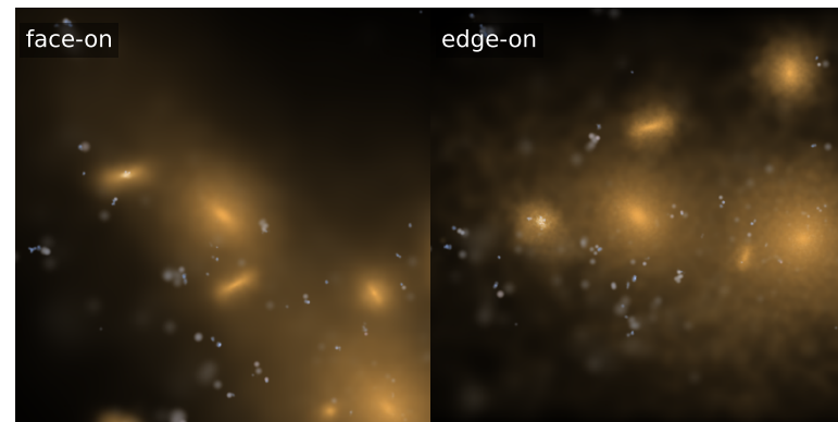
Subhalo 44523 [S] \log M_* = 10.97 DoR = 0.61 \log \Sigma_{1.5} = 10.01
