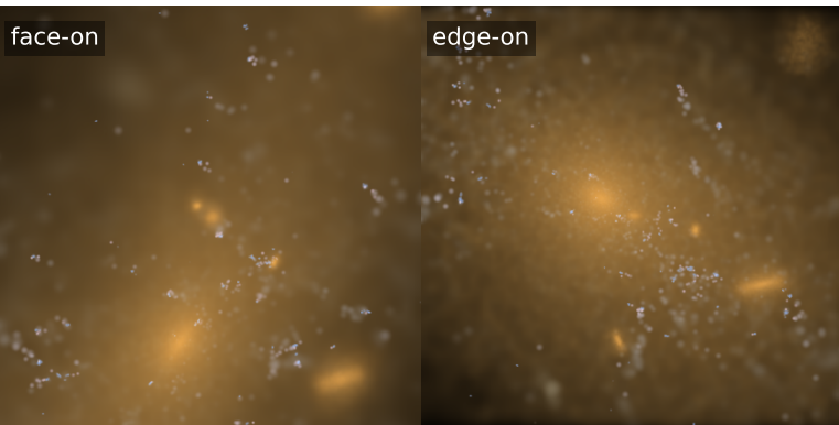
Subhalo 23328 [S] \log M_* = 10.17 DoR = 0.63 \log \Sigma_{1.5} = 9.87
