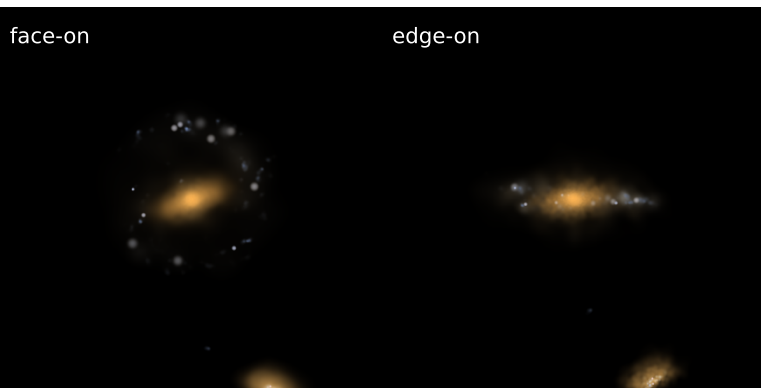
Subhalo 59531 [C] \log M_* = 10.57 DoR = 0.73 \log \Sigma_{1.5} = 10.17
