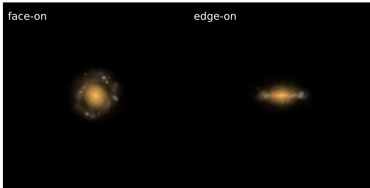
Subhalo 7997 [C] \log M_* = 10.46 DoR = 0.73 \log \Sigma_{1.5} = 9.80
