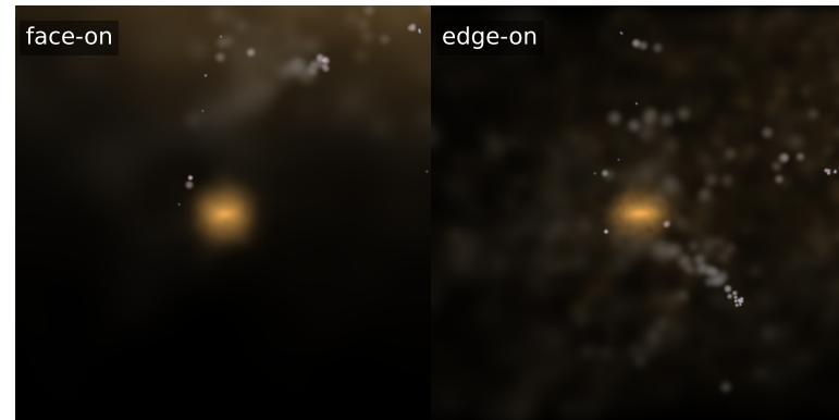
Subhalo 2348093 [S] \log M_* = 10.48 DoR = 0.67 \log \Sigma_{1.5} = 10.06
