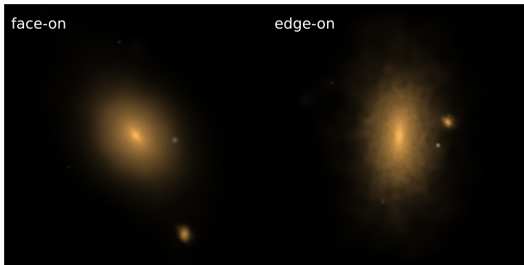
Subhalo 304 [C] \log M_* = 10.97 DoR = 0.65 \log \Sigma_{1.5} = 9.83
