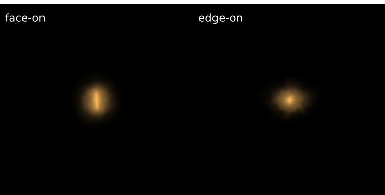
Subhalo 129078 [C] \log M_* = 10.52 DoR = 0.64 \log \Sigma_{1.5} = 9.91
