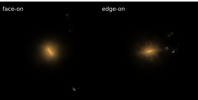
Subhalo 104782 [S] \log M_* = 10.84 DoR = 0.69 \log \Sigma_{1.5} = 10.38
