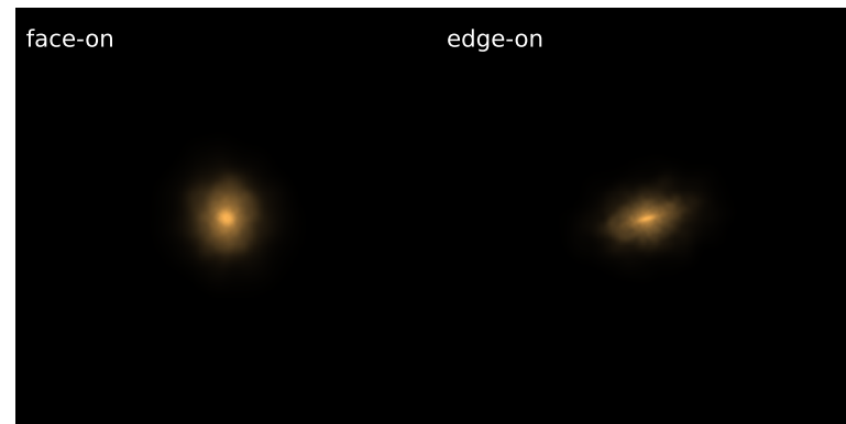
Subhalo 61127 [C] \log M_* = 10.64 DoR = 0.67 \log \Sigma_{1.5} = 10.43
