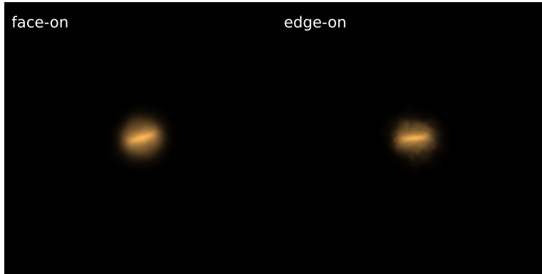
Subhalo 252431 [S] \log M_* = 10.45 DoR = 0.66 \log \Sigma_{1.5} = 9.86
