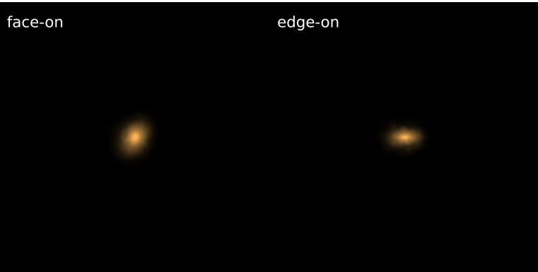
Subhalo 18408 [S] \log M_* = 10.28 DoR = 0.77 \log \Sigma_{1.5} = 10.06
