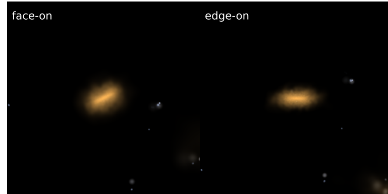
Subhalo 4323 [S] \log M_* = 10.50 DoR = 0.60 \log \Sigma_{1.5} = 9.78
