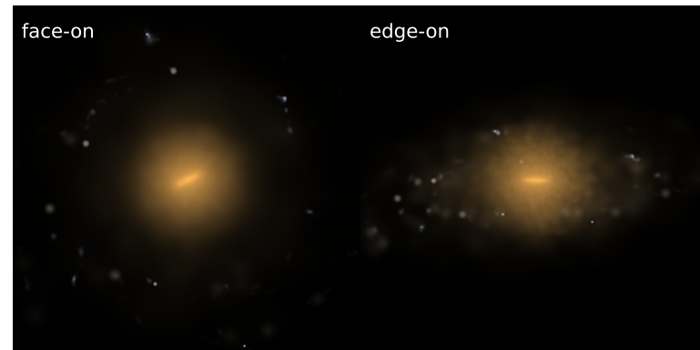
Subhalo 1415 [C] \log M_* = 11.08 DoR = 0.62 \log \Sigma_{1.5} = 10.17
