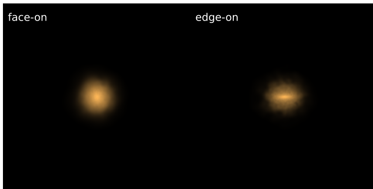
Subhalo 1867573 [S] \log M_* = 10.58 DoR = 0.65 \log \Sigma_{1.5} = 9.84
