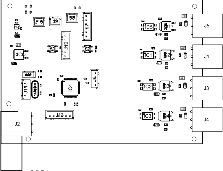
View from Top side (Scale 1:1)
