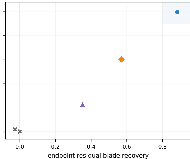
405B
