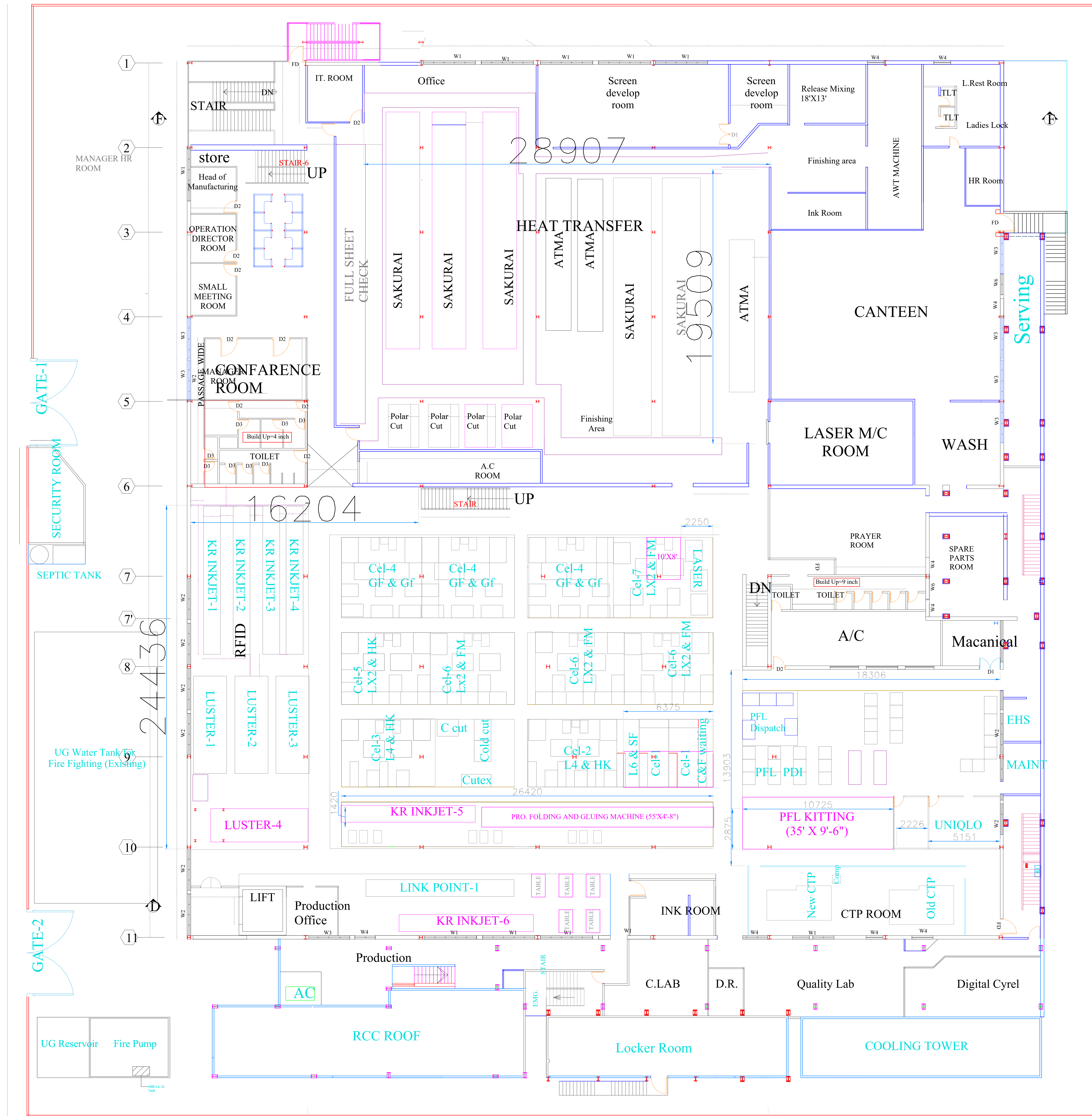
MACHINE LAYOUT PLAN (FF)
