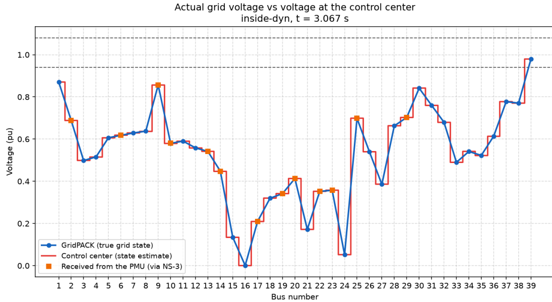
Figure 34. plot_profile.py on the dynamic IEEE 39 run, 67 ms after the three-phase fault at bus 16: bus 16 is at 0 pu, its neighbours between 0.1 and 0.6 pu; the PMU values and the estimate lie on the true curve.
