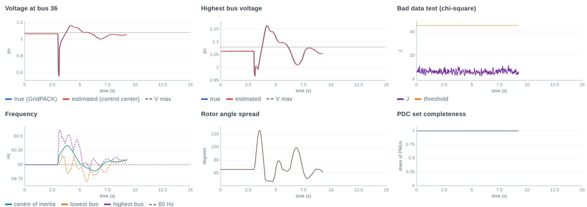
Figure 26. Live charts at 9.3 s: the fault at 3 s pulls bus 36 down to 0.56 pu; the exciters overshoot; frequency and rotor angles swing and settle.
