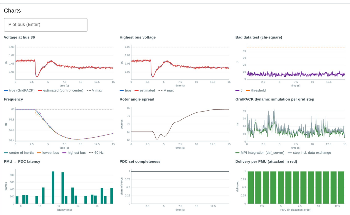
Figure 28. Results charts of the generator trip: frequency falls to 59.42 Hz and is arrested by the governors; GridPACK needs about 14 ms per frame on one rank.
