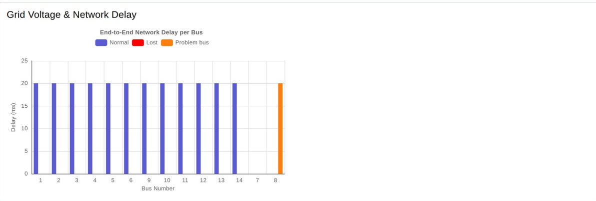
Figure 30. End-to-end network delay per bus. The voltage chart beside it loads its chart library from the internet and stays empty on servers without internet access.
