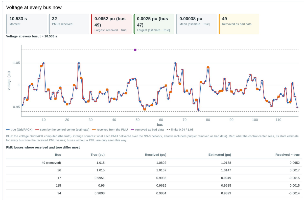
Figure 12. Voltage at every bus now, 10.5 s into an IEEE 118 run during a false data injection on bus 49: PMU 49 (purple) reports 1.080 pu for a true 1.015 pu; it is removed as bad data and the estimate (red) follows the truth (blue).
