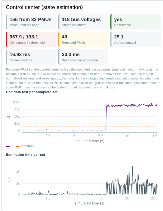
Fig. 6. Control-center panel of the Inside page during a simple FDI on bus 49.
