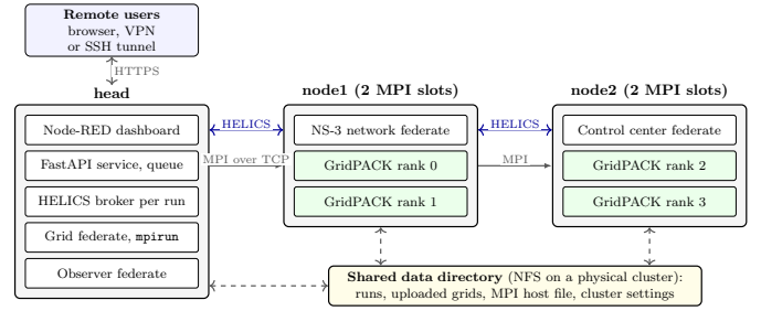
Fig. 7. Deployment on the three-node cluster.
