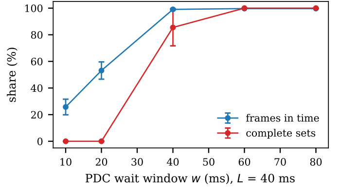
Fig. 15. Frames in time and complete sets against PDC wait window ( L = 40 ms).
