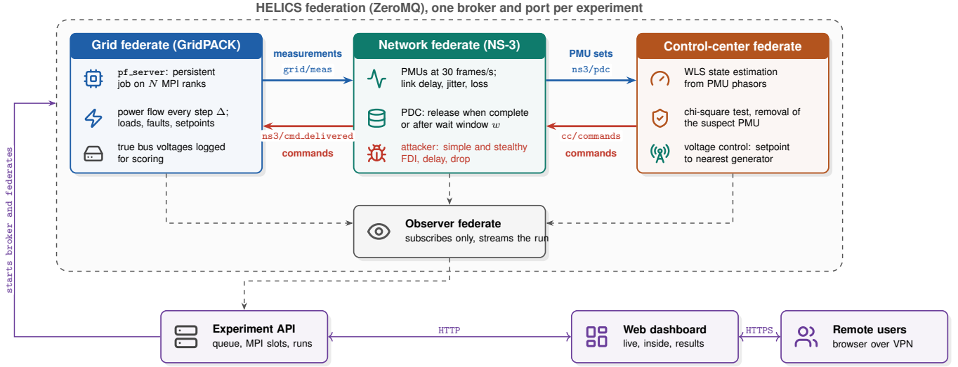
Fig. 1. Testbed architecture for one experiment.
