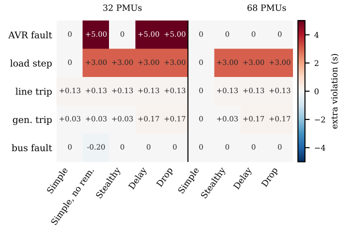
Fig. 13. Extra violation caused by each attack, per fault type (s).
