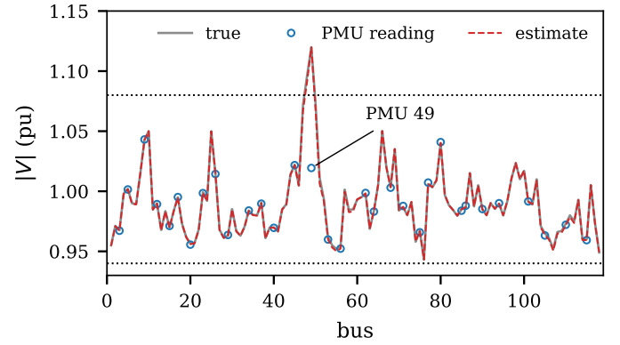
Fig. 12. Bus voltages in the set stamped 4.1 s, simple FDI on bus 49.
