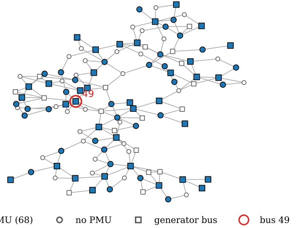
Fig. 3. Redundant placement, 68 PMUs.
