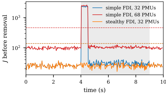
Fig. 11. Chi-square statistic J (solid) and threshold (dashed), seed 1.
