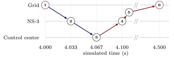
Fig. 4. Logged closed-loop timeline after the AVR fault at 4 s.
