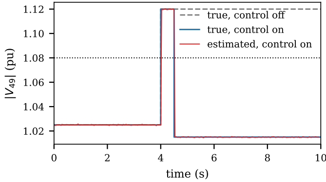
Fig. 8. Voltage of bus 49 with and without control (seed 1).
