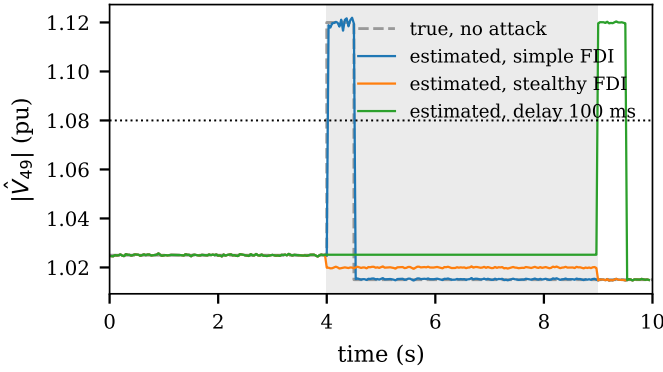
Fig. 10. Estimate of bus 49 under three attacks, 32 PMUs (seed 1).
