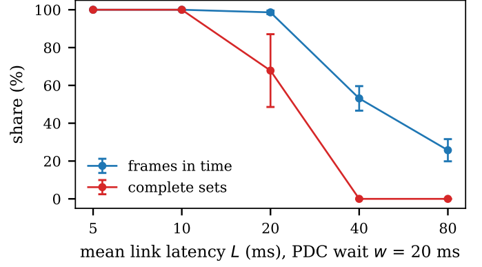
Fig. 14. Frames in time and complete sets against mean link latency ( w = 20 ms).
