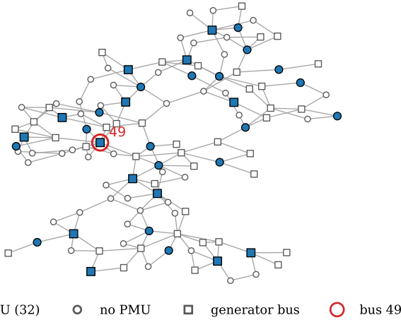
Fig. 2. Minimum placement, 32 PMUs.
