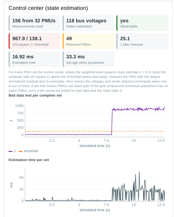
Fig. 8. Control-center panel of the Inside page during a simple FDI on bus 49.
