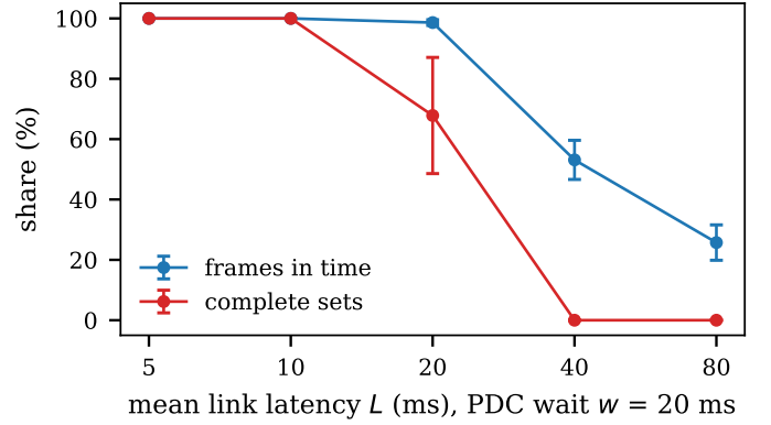
Fig. 21. Frames in time and complete sets against mean link latency ( w = 20 ms).
