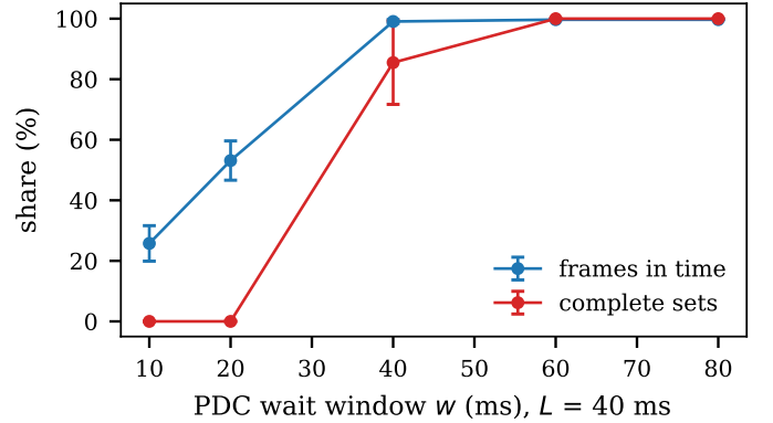
Fig. 22. Frames in time and complete sets against PDC wait window ( L = 40 ms).
