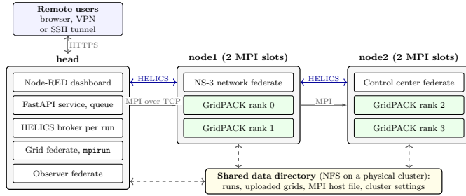
Fig. 9. Deployment on the three-node cluster.
