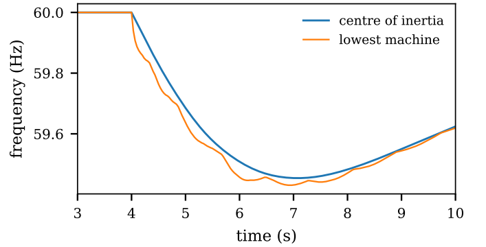
Fig. 19. Frequency after the trip of generator 80, with control (seed 1).
