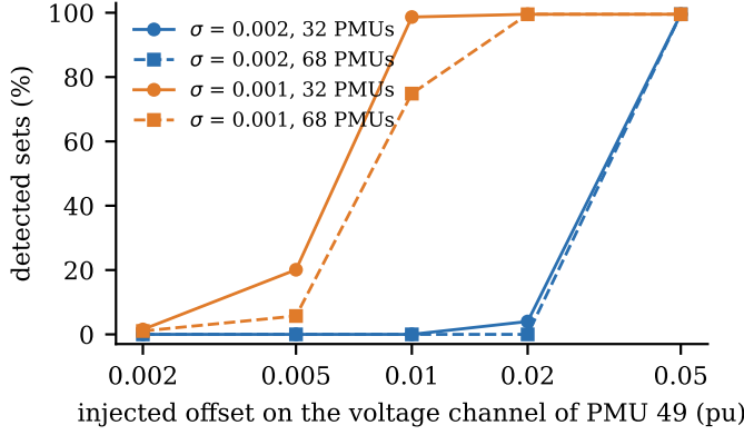
Fig. 20. Share of PDC sets in which the test detected a simple FDI, by offset size.
