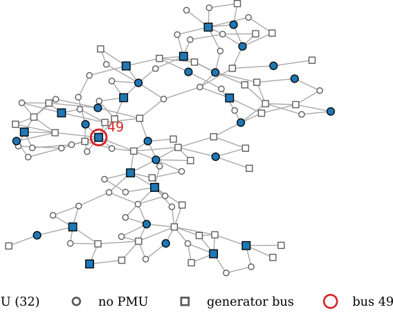
Fig. 4. Minimum placement, 32 PMUs.
