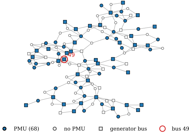
Fig. 5. Redundant placement, 68 PMUs.
