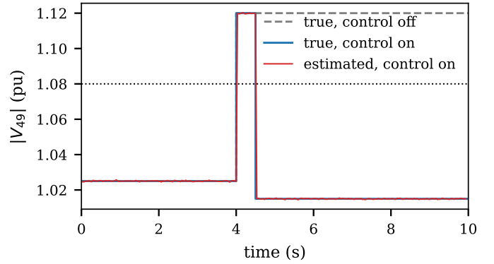
Fig. 10. Voltage of bus 49 with and without control (seed 1).
