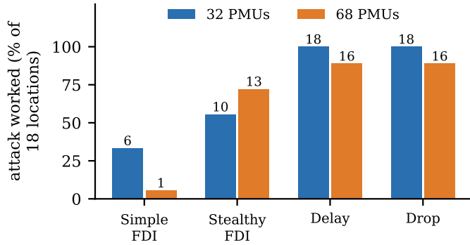
Fig. 16. Share of the 18 locations where each attack extended the violation.
