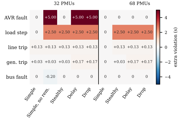
Fig. 15. Extra violation caused by each attack, per fault type (s).
