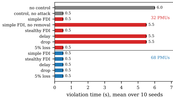
Fig. 11. Violation time per scenario, AVR fault (mean and 95% CI over ten seeds).
