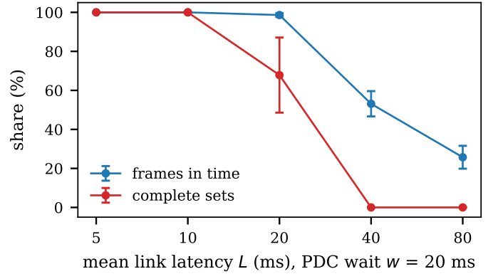
Fig. 20. Frames in time and complete sets against mean link latency ( w = 20 ms).
