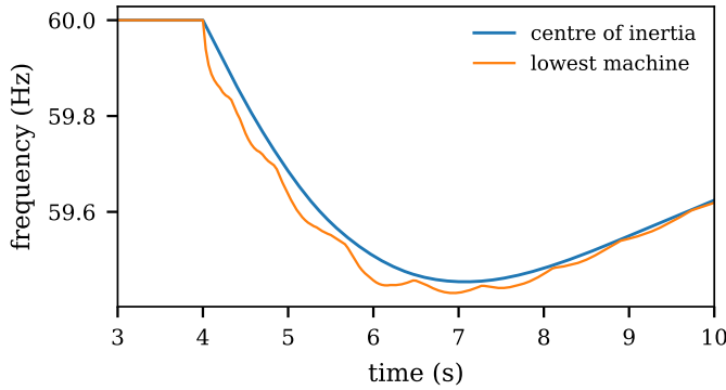
Fig. 19. Frequency after the trip of generator 80, with control (seed 1).
