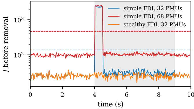
Fig. 13. Chi-square statistic J (solid) and threshold (dashed), seed 1.
