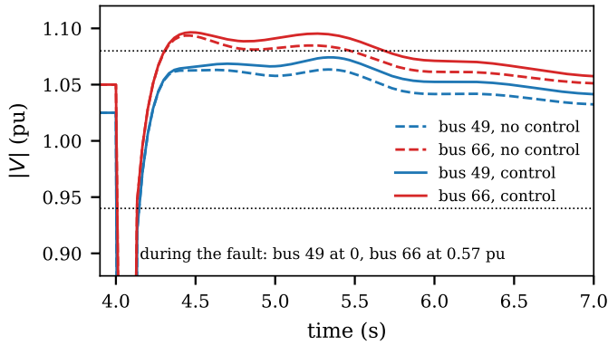
Fig. 17. Bus voltages around the three-phase fault at bus 49 (seed 1).
