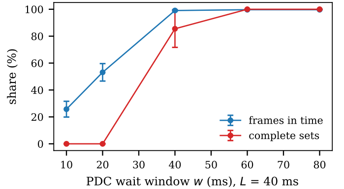
Fig. 21. Frames in time and complete sets against PDC wait window ( L = 40 ms).
