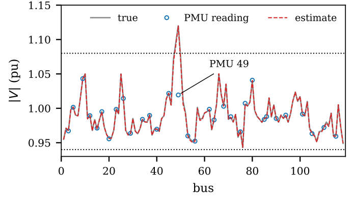
Fig. 14. Bus voltages in the set stamped 4.1 s, simple FDI on bus 49.
