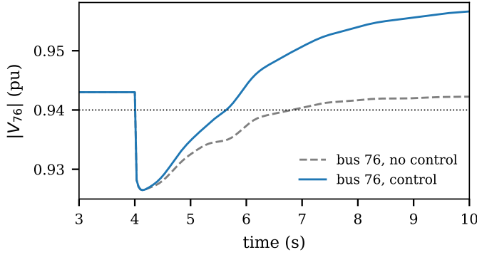
Fig. 18. Voltage of bus 76 after the trip of generator 80 (seed 1).
