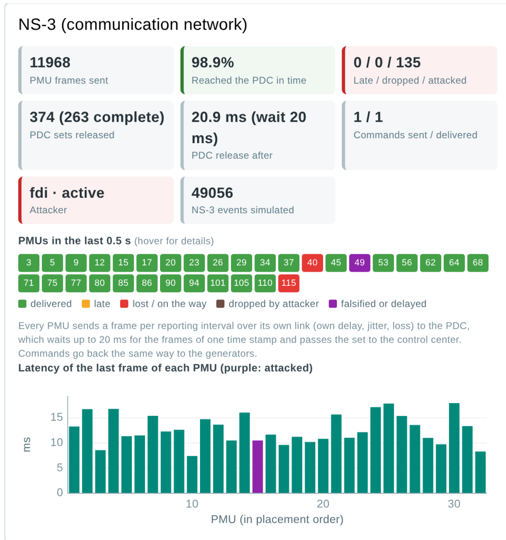
Figure 15. NS-3 panel: 98.9% of the frames arrive in time (1% loss: PMUs with a lost frame in the last 0.5 s are red); PMU 49 is attacked (purple); the PDC waits up to 20 ms for each set.
