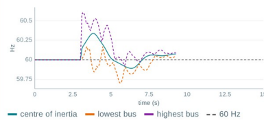
Figure 23. Live charts at 9.3 s: the fault at 3 s pulls bus 36 down to 0.56 pu; the exciters overshoot; frequency and rotor angles swing and settle.
