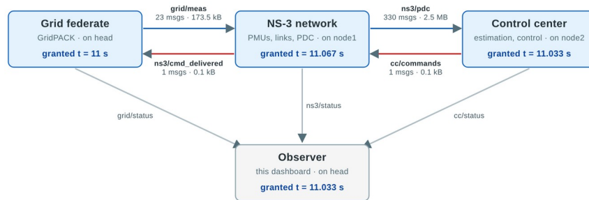
Figure 12. HELICS panel: grid federate on the head, NS-3 on node1, control center on node2, observer on the head, with their granted times; blue arrows carry measurements, red arrows commands, grey arrows copies for the dashboard.
