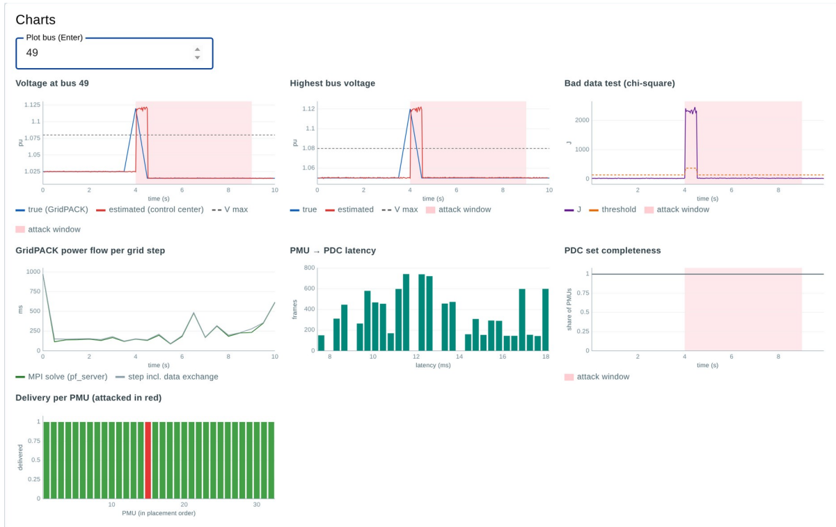
Figure 20. Result charts: voltage at bus 49, highest voltage, chi-square test, GridPACK solve time per grid step, PMU-to-PDC latency, PDC completeness and delivery per PMU (attacked PMU in red).
