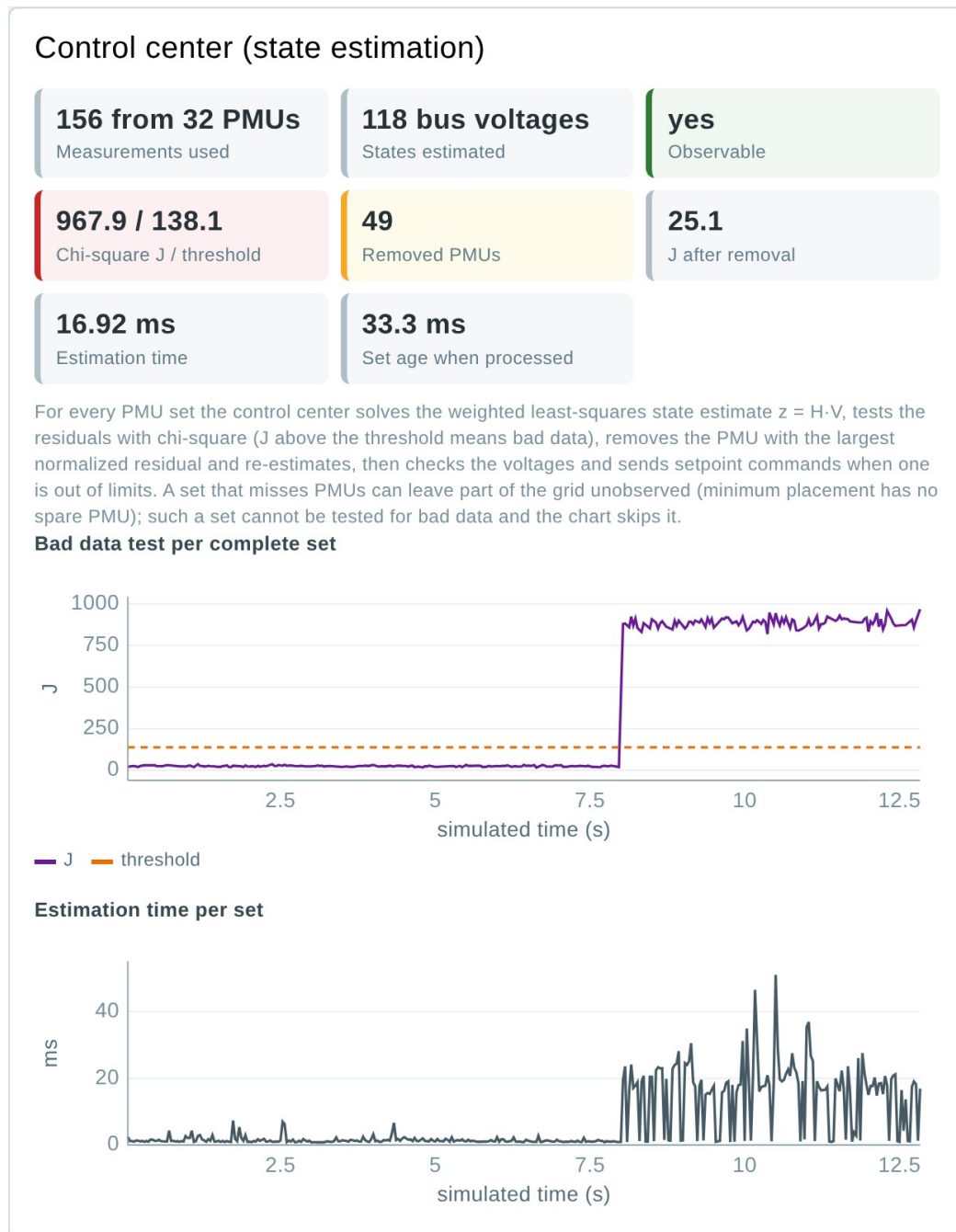
Figure 16. Control center panel: during the attack J is about 900 against a threshold of 138; PMU 49 is removed and J falls to 25; with the residual test and the second estimate a set takes 10-40 ms instead of about 1 ms.
