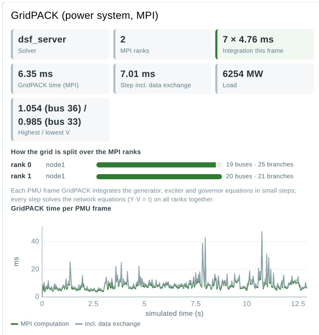
Figure 14. GridPACK panel in dynamic mode (IEEE 39, fault at bus 16 at 3 s): 7 integration steps of 4.76 ms per PMU frame, 6-10 ms of MPI time per frame.
