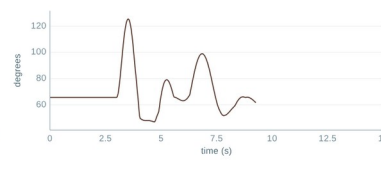
Figure 23. Live charts at 9.3 s: the fault at 3 s pulls bus 36 down to 0.56 pu; the exciters overshoot; frequency and rotor angles swing and settle.
