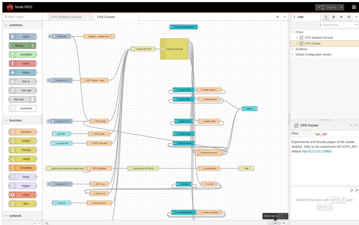
Figure 30. The CPS Cluster flow in the Node-RED editor.
