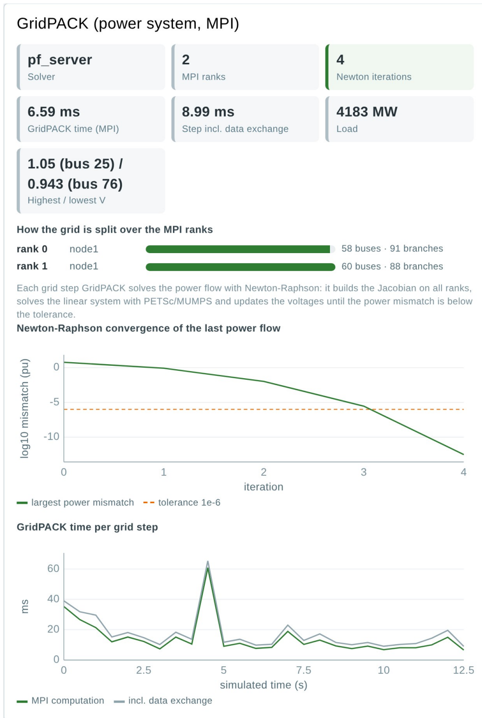
Figure 13. GridPACK panel in power flow mode: 2 ranks on node1 with 58 and 60 buses; Newton-Raphson needs 4 iterations, the mismatch falls from 5.9 to 3 \times 10^{-13} pu.
