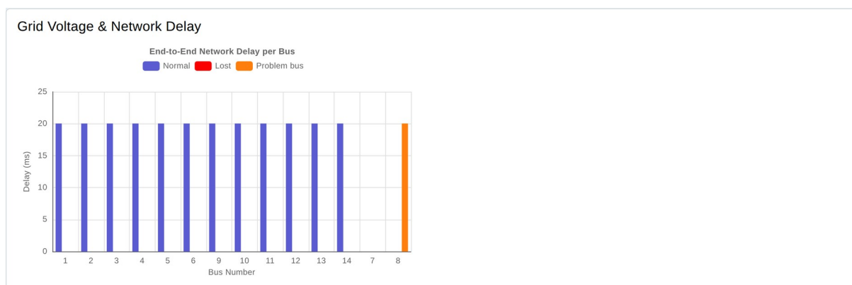
Figure 27. End-to-end network delay per bus. The voltage chart beside it loads its chart library from the internet and stays empty on servers without internet access.
