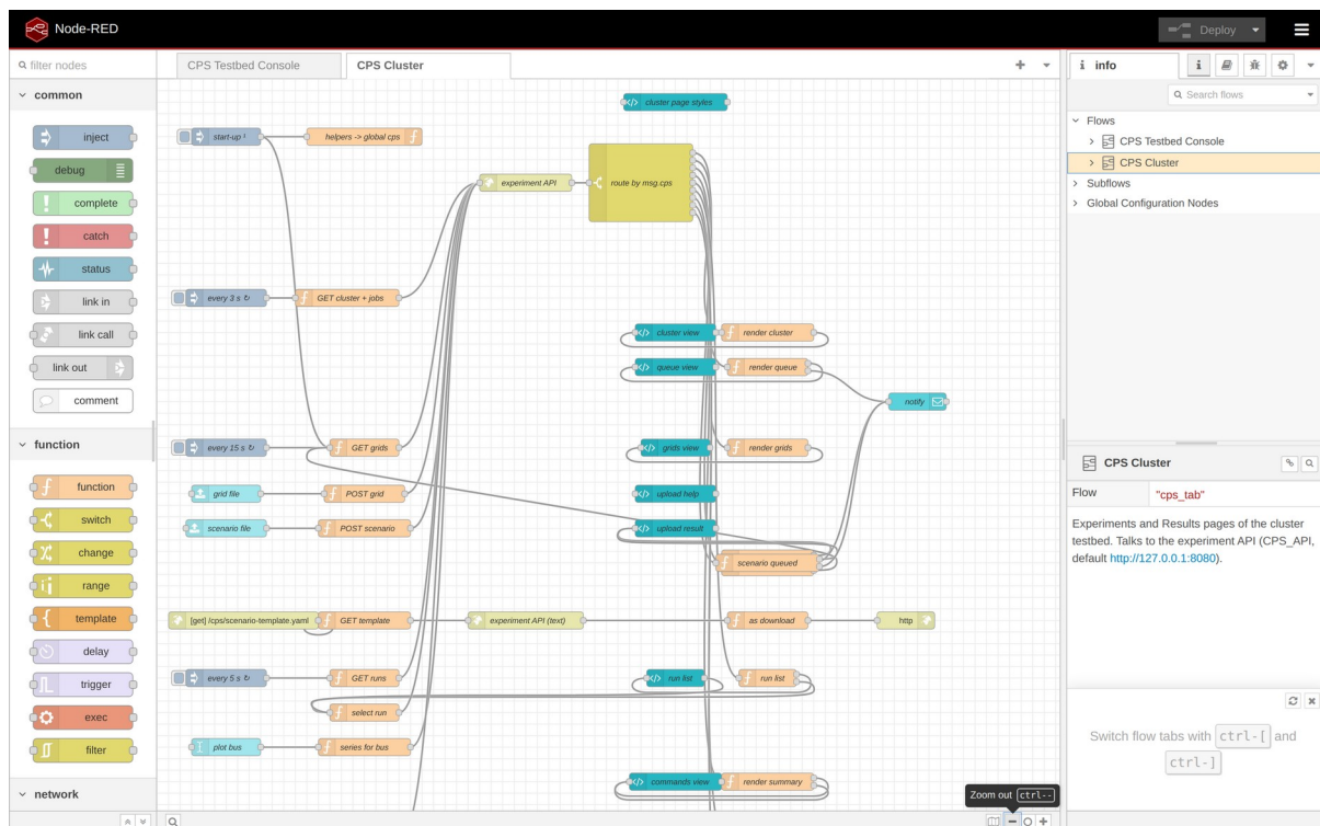
Figure 18. The CPS Cluster flow in the Node-RED editor.
