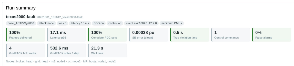
Figure 19. Summary of the 2000-bus run on the cluster.
