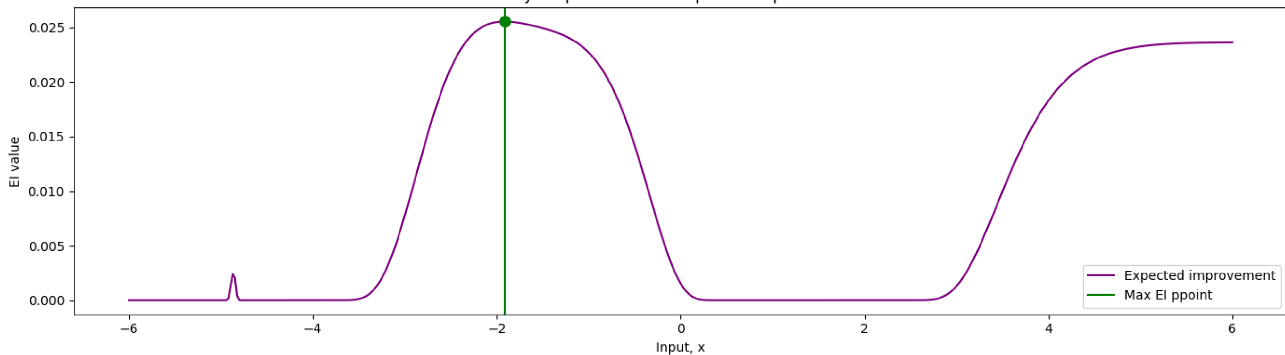
Bayes opt iteration 4: Expected improvement
