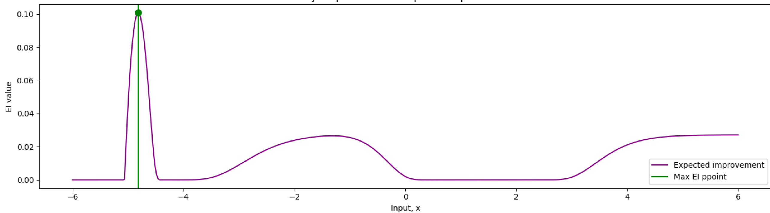
Bayes opt iteration 3: Expected improvement
