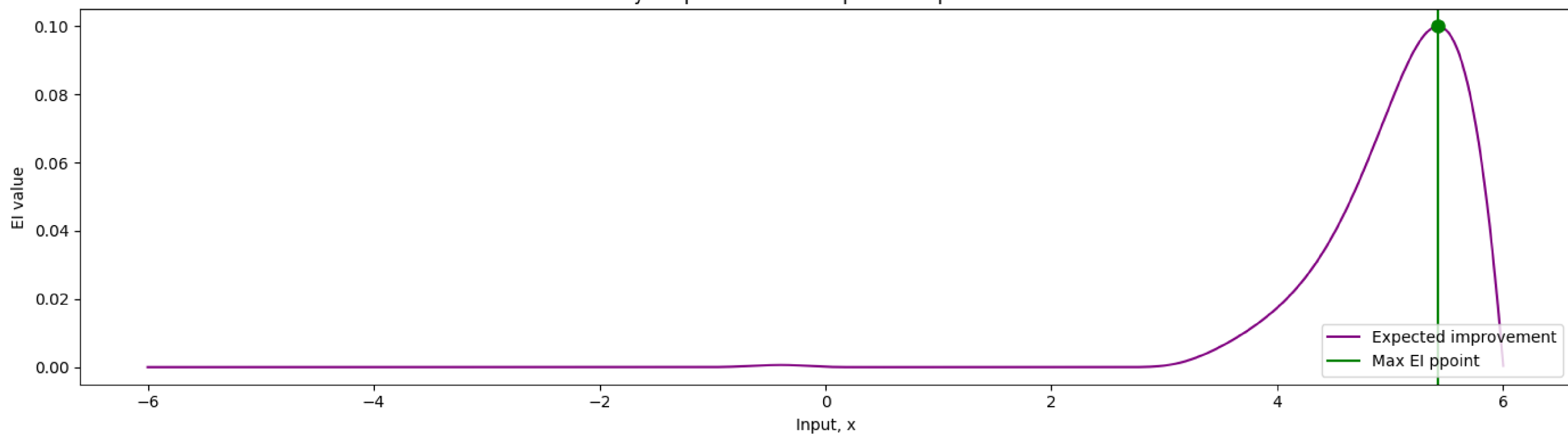
Bayes opt iteration 6: Expected improvement
