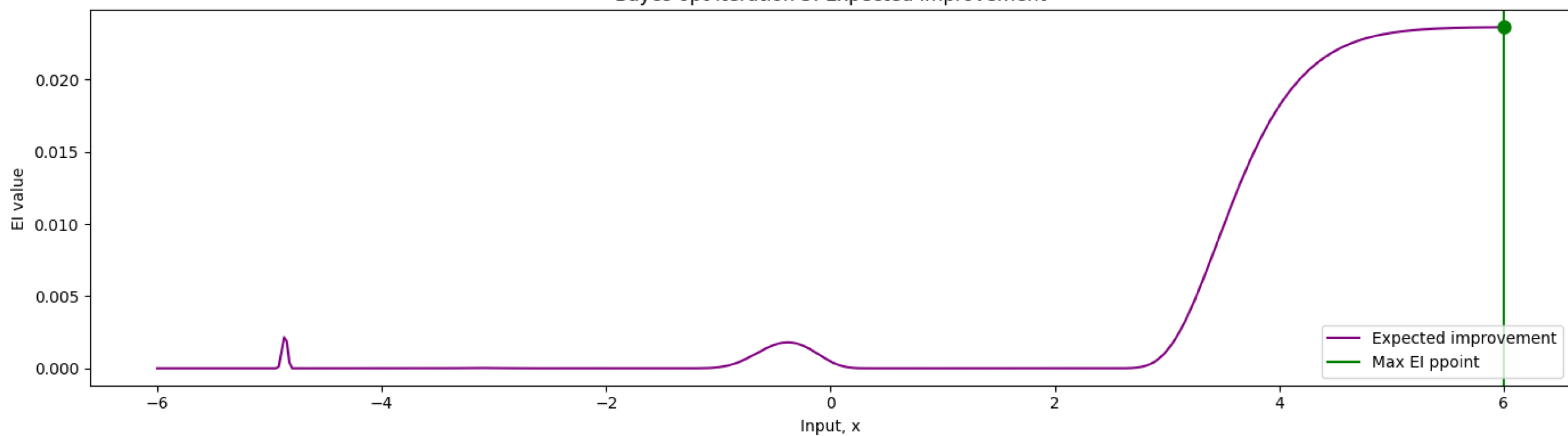
Bayes opt iteration 5: Expected improvement
