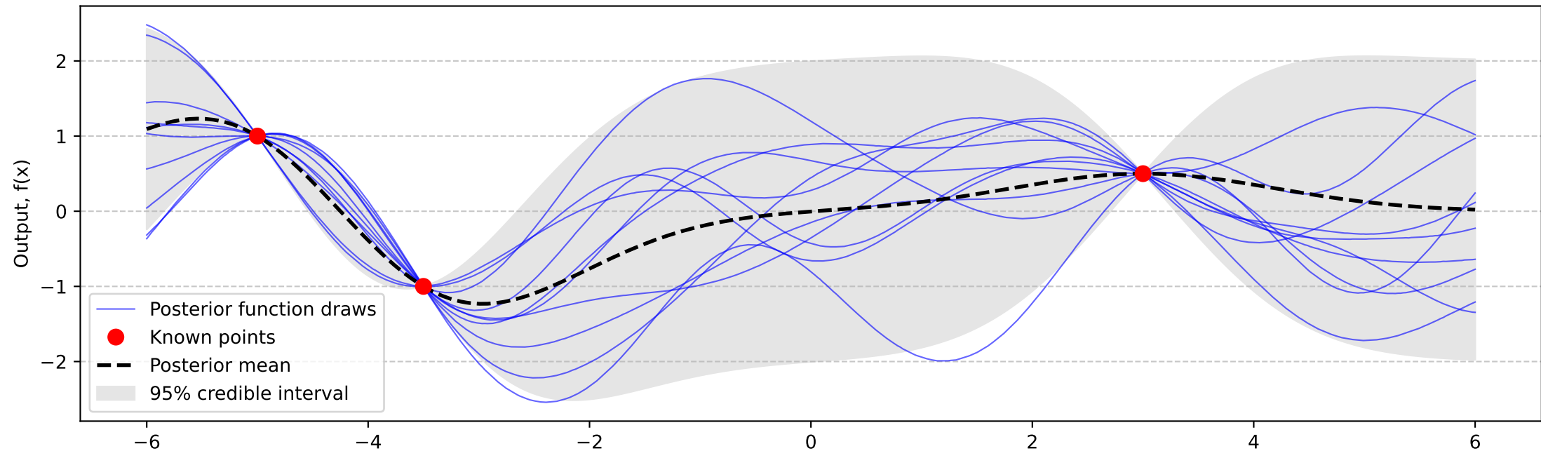
Gaussian process posterior and samples
