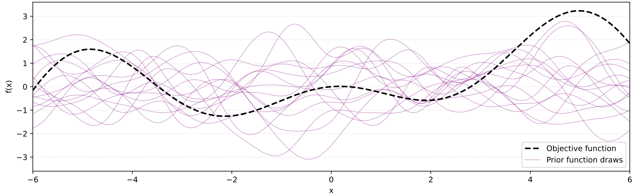
Gaussian process prior and objective function
