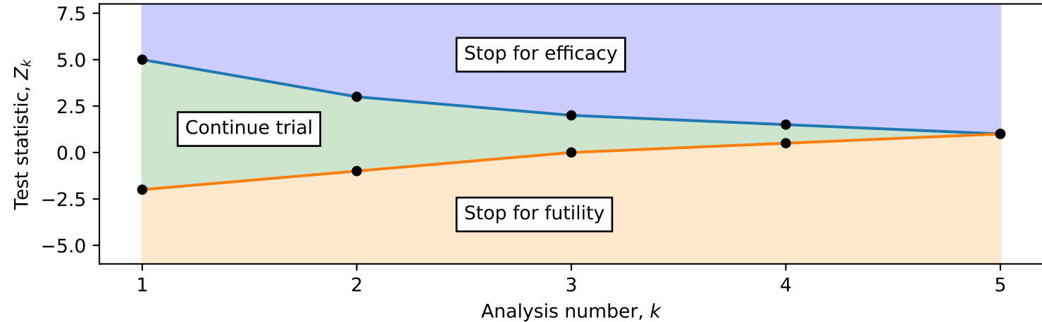
Group sequential bounds for a 5-stage design
