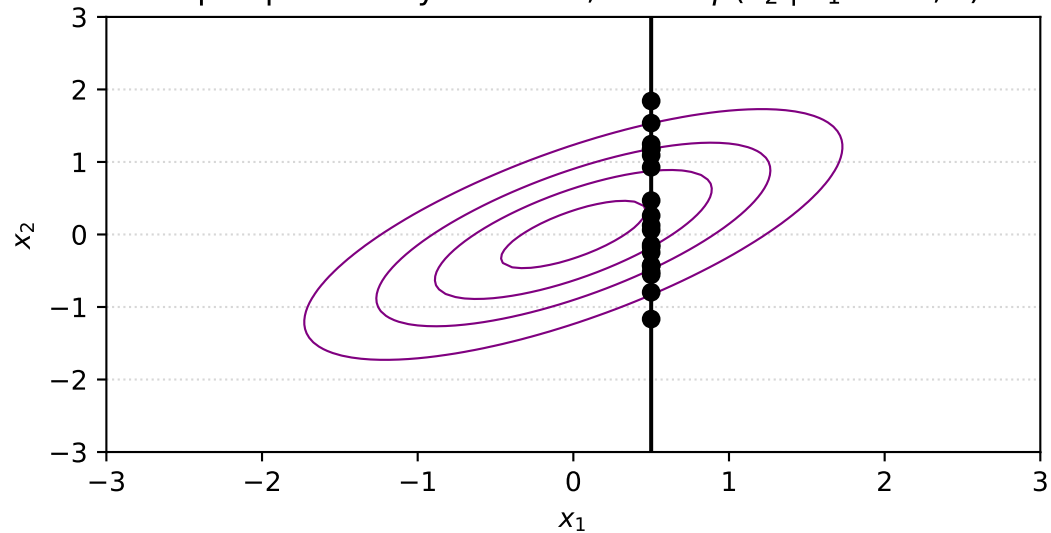
Equal probability contours, draws p(x_2 | x_1 = 0.5, \Sigma)
