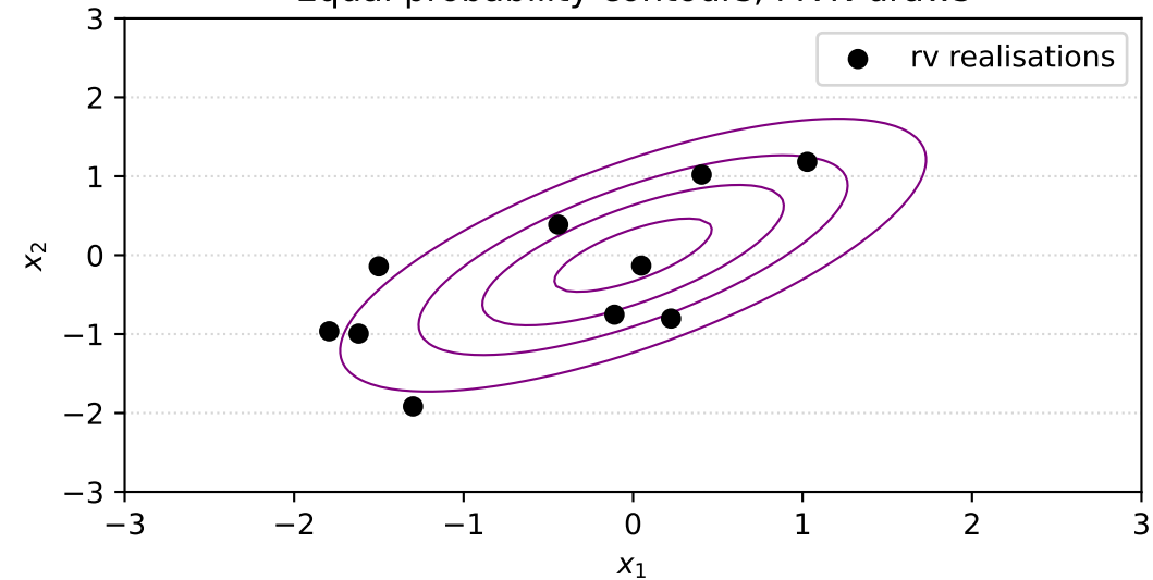
Equal probability contours, MVN draws
