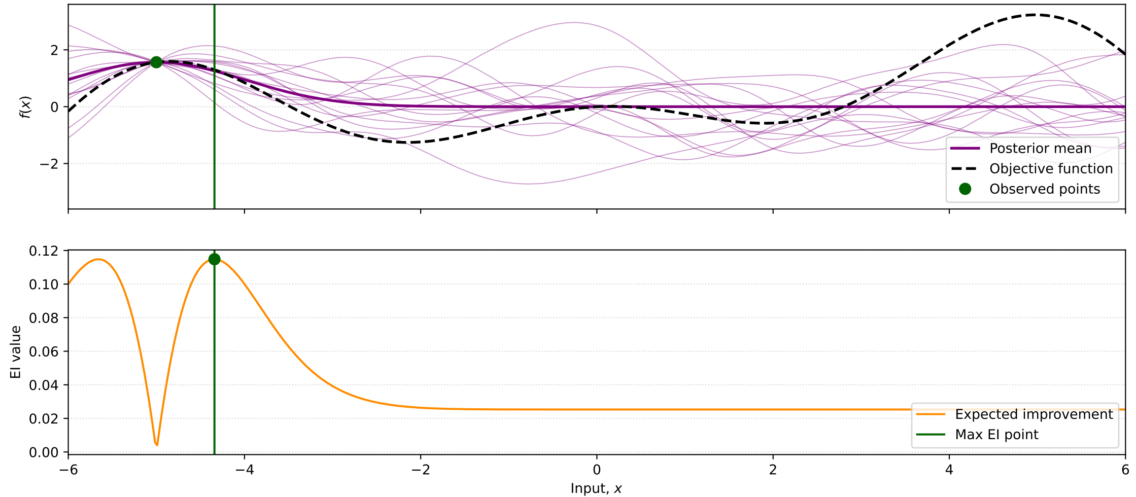
Bayes opt iteration 1: Gaussian process fit, objective function, and expected improvement
