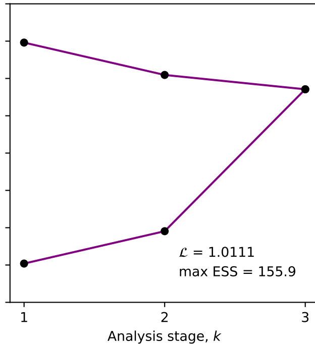
O'Brien-Fleming boundaries
