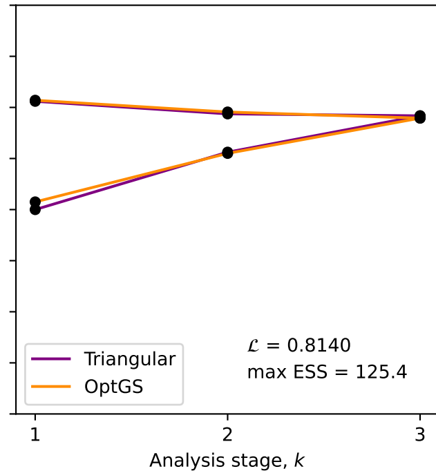
Triangular and OptGS boundaries
