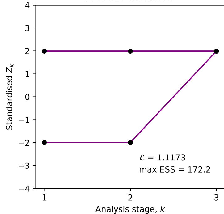
Pocock boundaries
