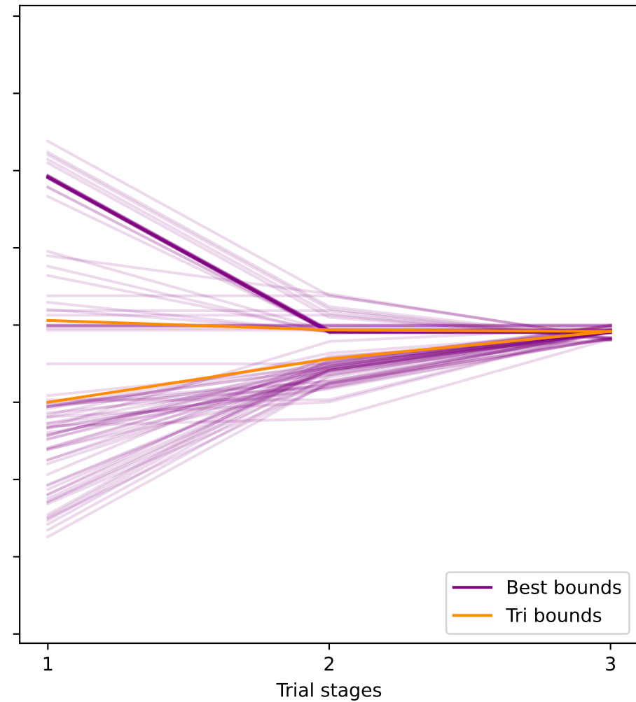
Bayesian optimisation, top 50 bounds
