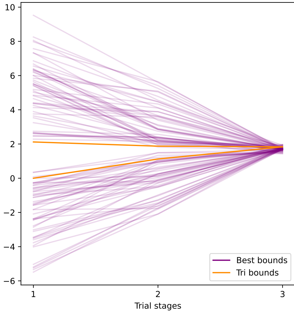
Random search, top 50 bounds
