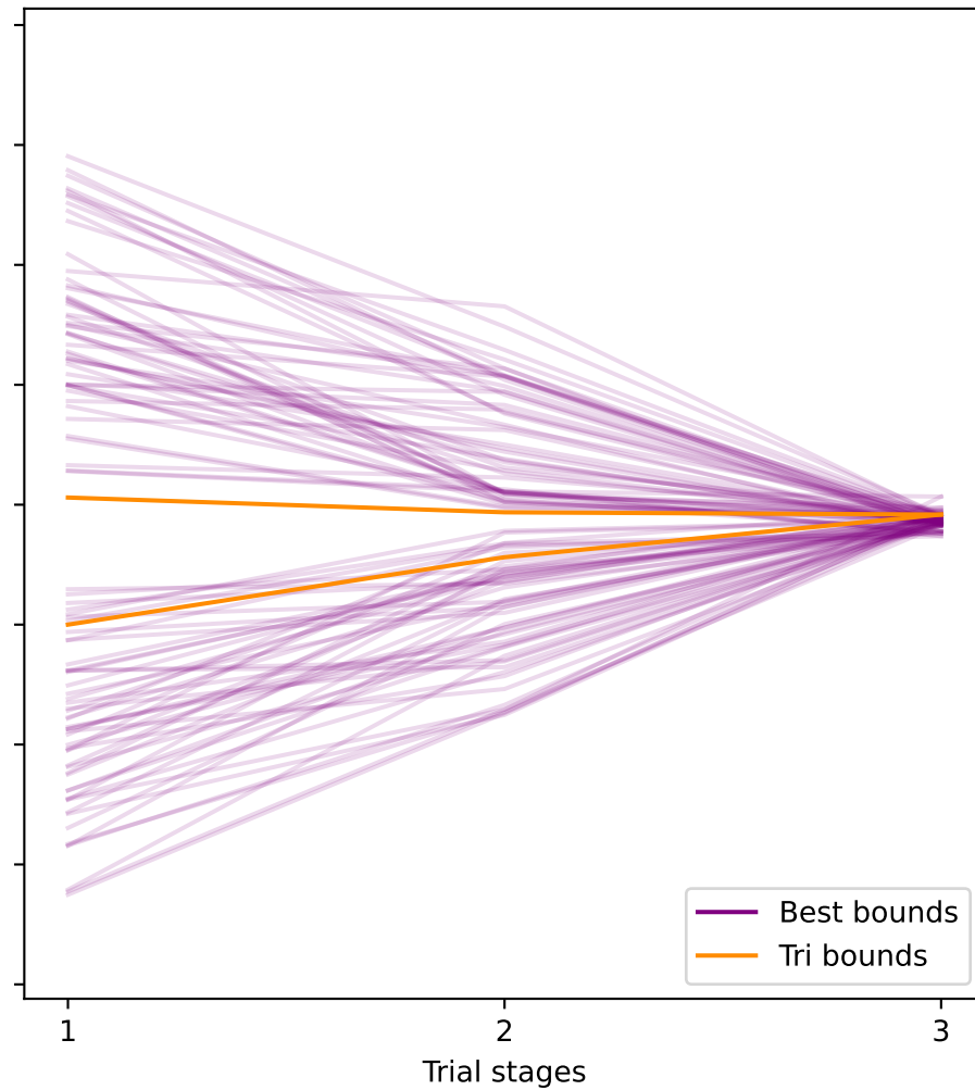
Simulated annealing, top 50 bounds
