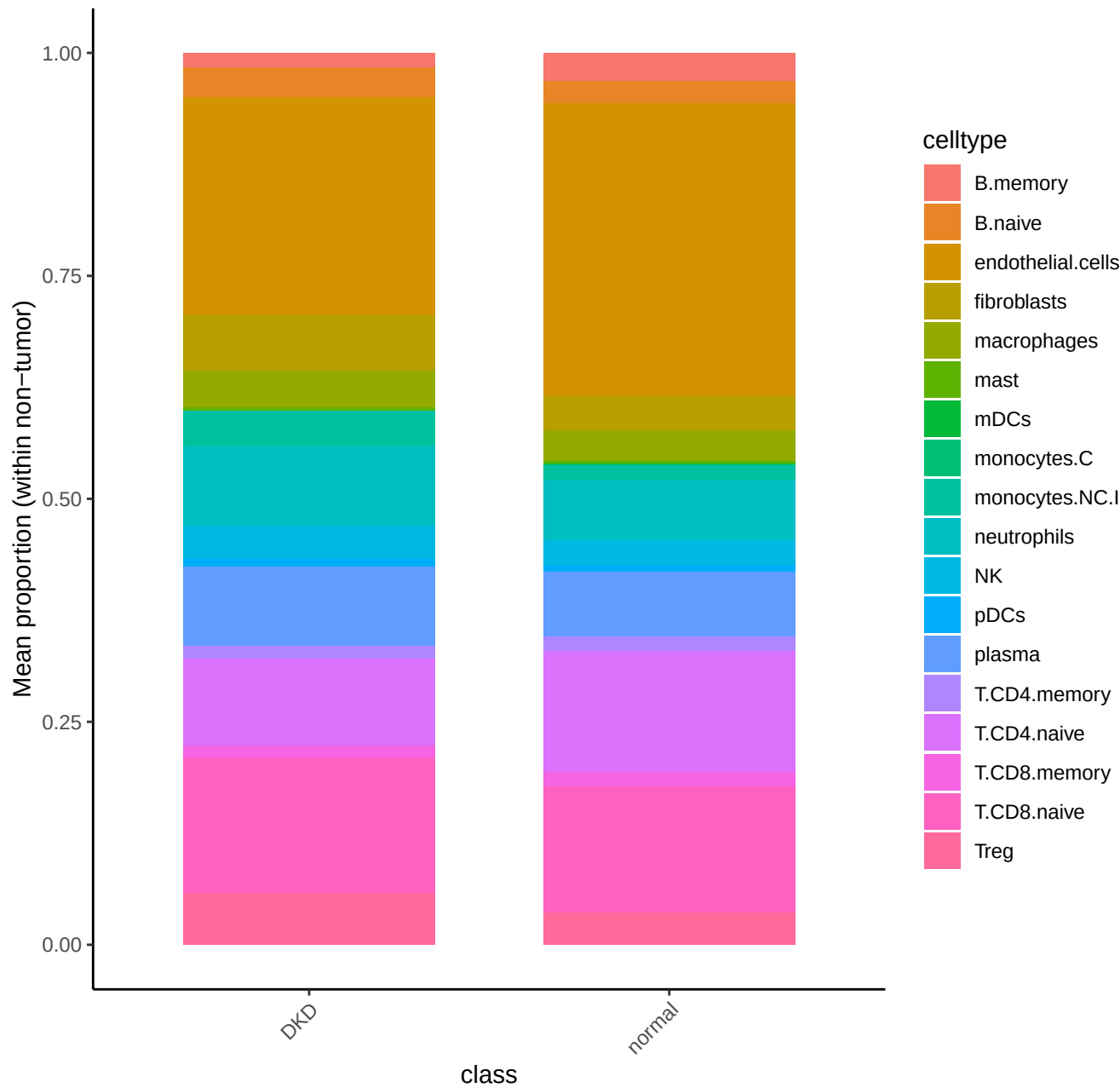
Cell-type composition by class (SpatialDecon)
