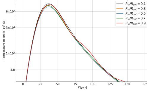
(a) R_{in,0}/R_{out,0} . Fijamos el valor de R_{out,0} = 150 R_g .
