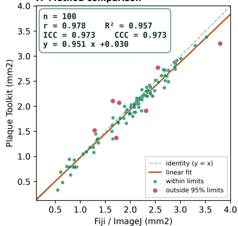
A Method comparison
