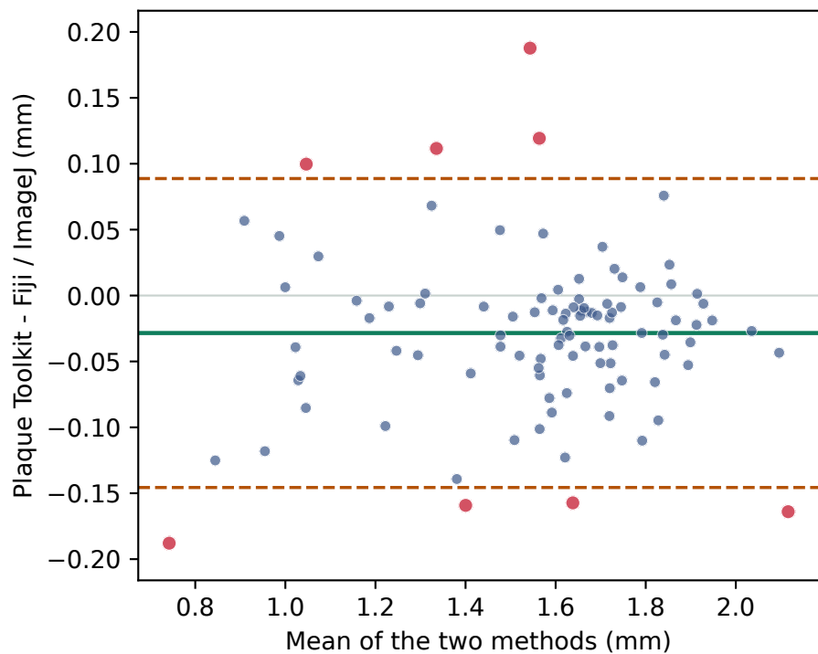
B Bland-Altman
