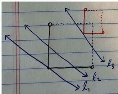
Figure 30: We can construct an open set [a, b) \times [c, d) where the point (a, c) lies on any point on a negatively sloping line. This means that points are open sets, which generates the discrete topology.
