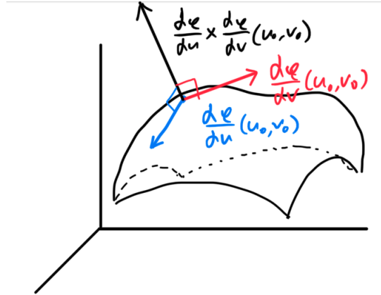
Figure 24: Note that the cross product \frac{\partial \varphi}{\partial u}(u_0, v_0) \times \frac{\partial \varphi}{\partial v}(u_0, v_0) \neq 0 if and only if D\varphi(u_0, v_0) is full rank, i.e. the tangent plane exists.
