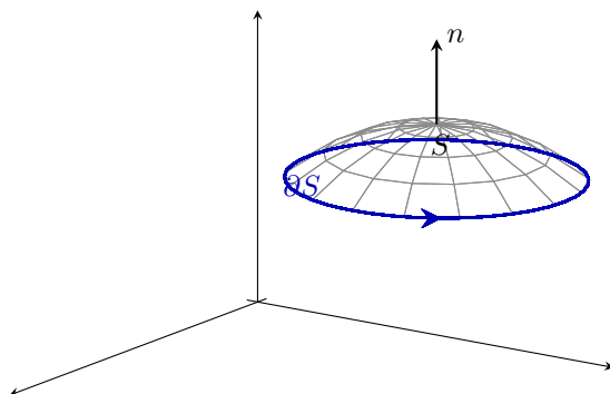
Figure 30: The orientation unit vector n of S induces the positive orientation of \partial S , denoted \partial S^+ . Visually, if you are walking along the curve with your head is pointing in the same direction as the unit normal vectors while the surface is on the left then you are walking in the positive direction on \partial S .
