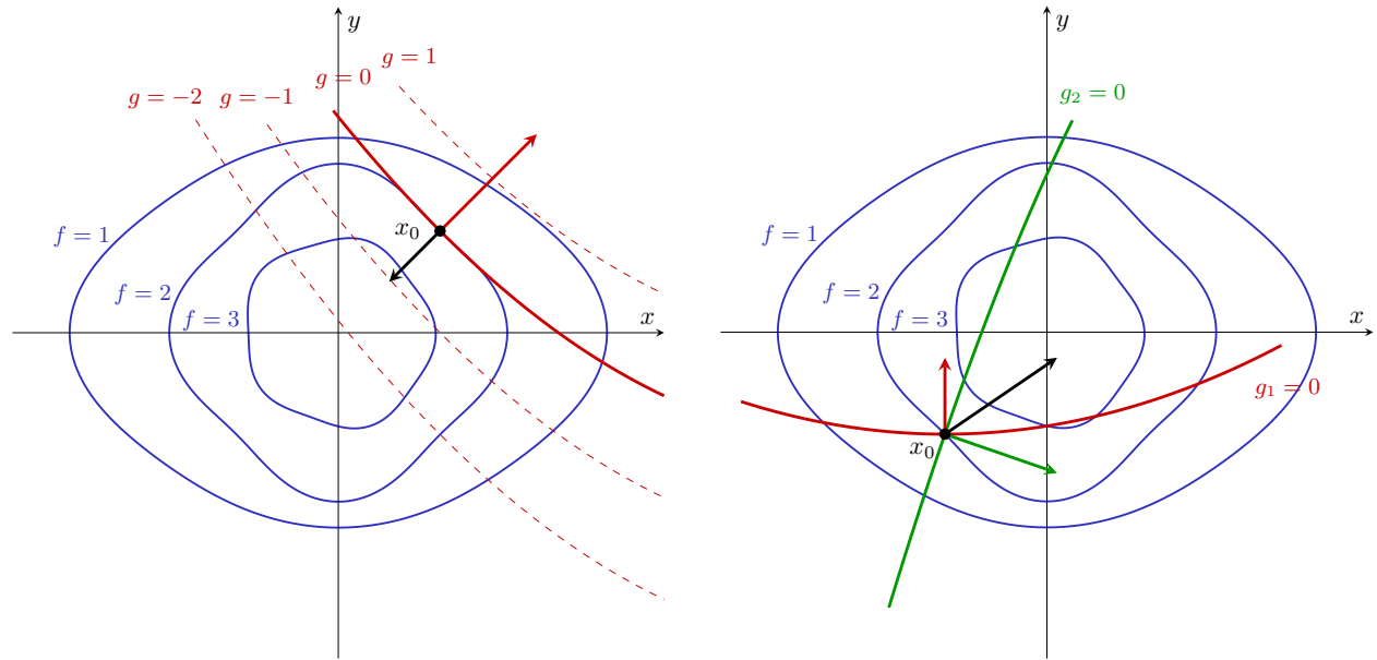
(a) When there is a single constraint g : \mathbb{R}^n \rightarrow \mathbb{R} , \nabla f(x_0) can be expressed as a linear combination of \nabla g(x_0) .
