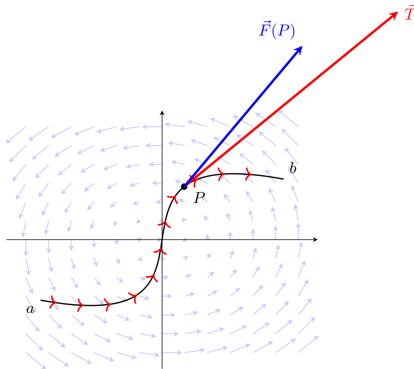
Figure 26: Visualizing a path integral. At a specific point P along the oriented curve, the red tangent vector \vec{T} points along the path, while the solid blue vector \vec{F}(P) represents the local vector field at that exact location. The path integral \int_C \vec{F} \cdot d\vec{r} accumulates the dot product of these two vectors at every point along the curve.
