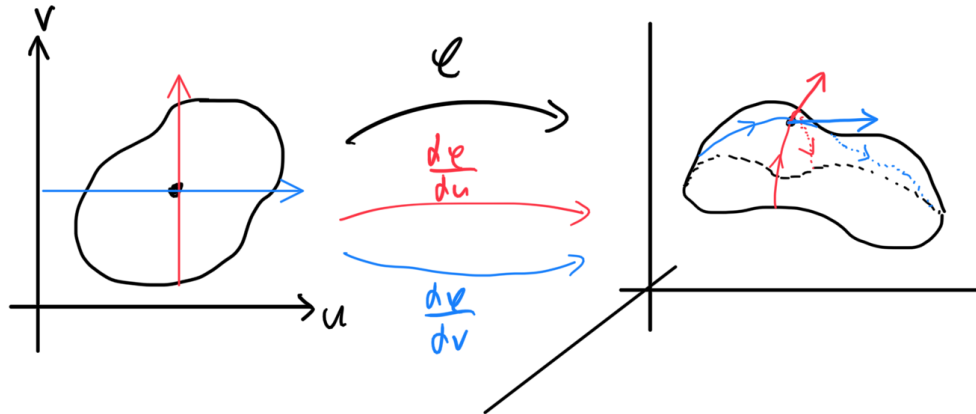
Figure 23: When \varphi : D \subset \mathbb{R}^2 \rightarrow \mathbb{R}^3 , we can see visually that given (u_0, v_0) \in D , there should be two linearly independent tangent vectors T_u, T_v sticking out from \varphi(u_0, v_0) on the surface E . So every vector in the “tangent plane” should be a linear combination of T_u and T_v . In fact, these two vectors are precisely T_u = \frac{\partial \varphi}{\partial u}(u_0, v_0) and T_v = \frac{\partial \varphi}{\partial v}(u_0, v_0) , so the tangent plane is really just \varphi(u_0, v_0) plus the vectors in the column space of D\varphi(u_0, v_0) !
