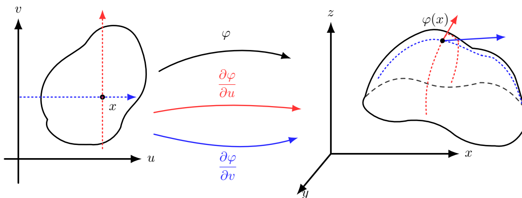
Figure 24: When \varphi : D \subset \mathbb{R}^2 \rightarrow \mathbb{R}^3 , we can see visually that given (u_0, v_0) \in D , there should be two linearly independent tangent vectors T_u, T_v sticking out from \varphi(u_0, v_0) on the surface E . So every vector in the “tangent plane” should be a linear combination of T_u and T_v . In fact, these two vectors are precisely T_u = \frac{\partial \varphi}{\partial u}(u_0, v_0) and T_v = \frac{\partial \varphi}{\partial v}(u_0, v_0) , so the tangent plane is really just \varphi(u_0, v_0) plus the vectors in the column space of D\varphi(u_0, v_0) !
