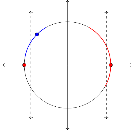
Figure 8: Let f : \mathbb{R}^2 \rightarrow \mathbb{R} be defined by f(x, y) = x^2 + y^2 - 1 . The level set at z = 0 would be the set of points satisfying x^2 + y^2 - 1 = 0 , i.e. the unit circle. The derivative of f with respect to y is 0 at the points (-1, 0) and (1, 0) , meaning that in any neighborhood of these points, we cannot define a function of y with respect to x . This is true, indeed, since any such function would fail the vertical line test, which can be seen in the red neighborhood around (1, 0) . However, the blue neighborhood of the point (-\sqrt{2}/2, \sqrt{2}/2) does indeed define a function of y with respect to x satisfying the vertical line test.
