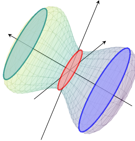
Figure 16: Visual of Cavalieri's principle.
