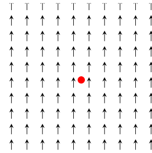
(c) \nabla \cdot \mathbf{F} = 0 (Constant)
