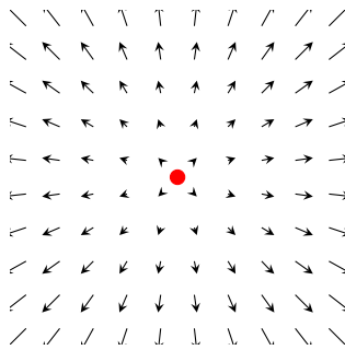
(a) \nabla \cdot \mathbf{F} > 0 (Source)
