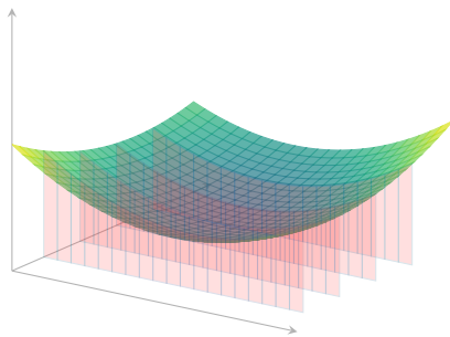
(a) Slicing at fixed values of y .
