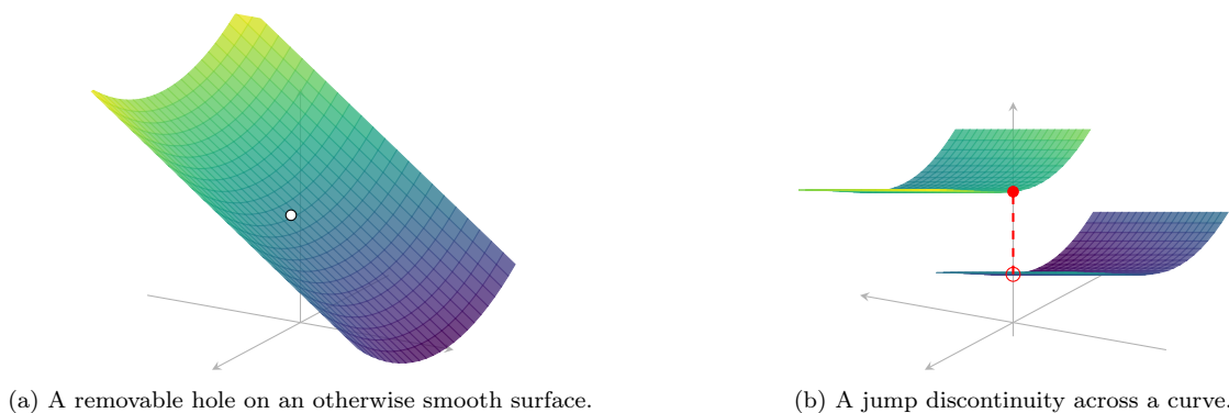
Figure 15: Two typical discontinuities that can still occur in integrable functions: a removable hole and a jump discontinuity.
