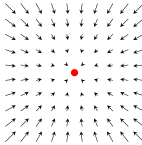
(b) \nabla \cdot \mathbf{F} < 0 (Sink)
