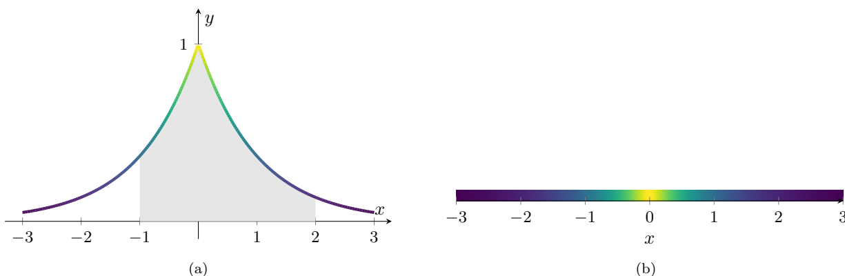
Figure 13: Two interpretations of the integral \int_{-1}^2 e^{-|x|} dx . On the left, we view it as the area under a curve. On the right, we view it as the mass of a 1-dimensional rod lying on [-1, 2] of varying density defined by function f(x) .
