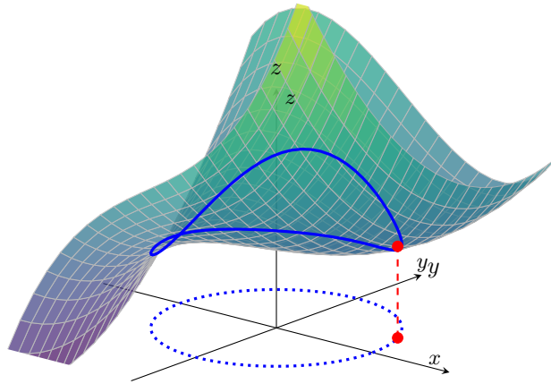
Figure 9: An example of a function f : \mathbb{R}^2 \rightarrow \mathbb{R} constrained to the unit circle, where g(x, y) = x^2 + y^2 - 1 = 0 . The blue curve in the xy -plane is the constraint set, and the upper blue curve is its image on the graph of f .
