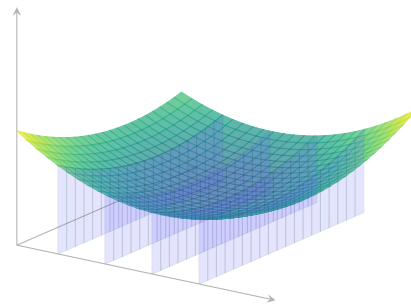
(b) Slicing at fixed values of x .
