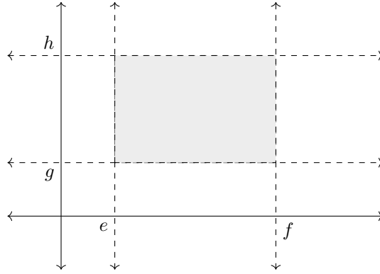
Figure 14: Visually, we can interpret each \mathcal{S}(U_\beta) as a "strip" in the total product space. For example in \mathbb{R}^2 , there are two "strips" (e, f) \times \mathbb{R} and \mathbb{R} \times (g, h) that intersect. Note that each strip is the preimage of the projection mapping.
