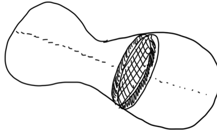
Figure 8: Visual of Cavalieri's principle.
