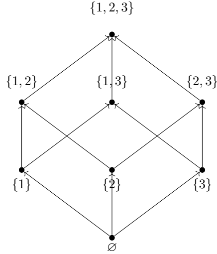
Figure 1: A finite category induced by a partial order. Identity morphisms and arrows obtained by composition are omitted.
