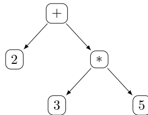
Figure 4: Syntax tree for the expression 2 + 3 * 5 .
