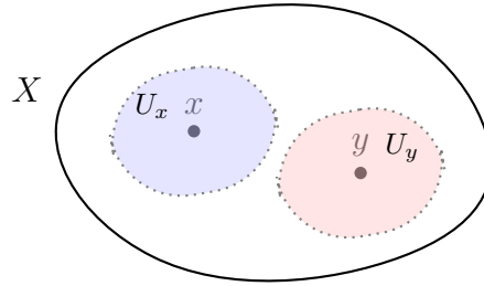
Figure 44: Every pair of distinct points must satisfy this separability condition in a Hausdorff space.
