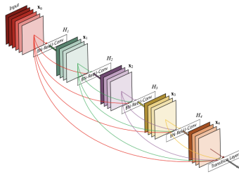
Figure 8: Densenet architecture.
