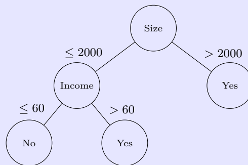
(b) The accuracy of this tree is 12 out of 12.
