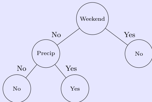
(a) The accuracy of this tree is 7 out of 12.
