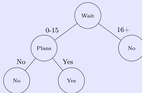
(b) The accuracy of this tree is 9 out of 12.
