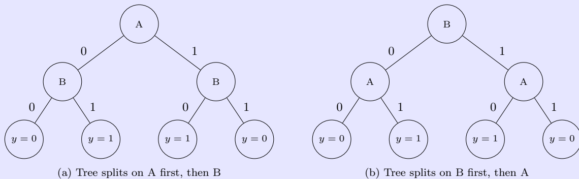
Figure 7: Two functionally equivalent decision trees that implement the XOR function: y = A \oplus B
