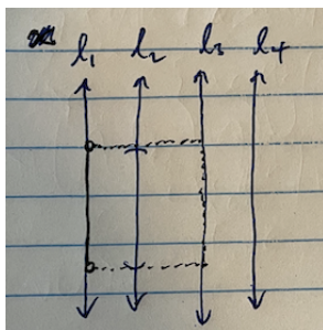
Figure 28: \ell_1, \ell_2 intersect the open set at open intervals. \ell_3, \ell_4 does not but there are always open sets for which the intersection are open intervals.
