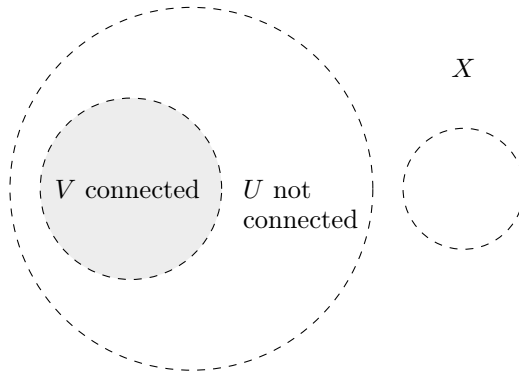
Figure 40: Visually, in the space X , let U be the union of the two open balls shown below. U is clearly open, but not necessarily connected. However, we can form a neighborhood V of x contained in U such that V is connected.
