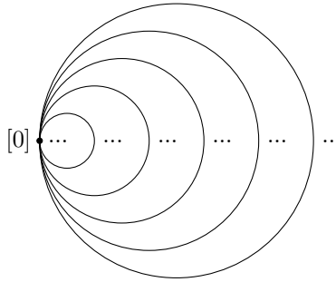
Figure 26: It turns out that every interval [j, j+1] \subset \mathbb{R} , j \in \mathbb{Z} will get mapped as a closed loop in \mathbb{R}/\sim beginning and ending with [0] , since j, j+1 \mapsto [0] . So geometrically, \mathbb{R}/\sim consists of an infinite number of nonintersecting closed loops starting and ending with [0] .
