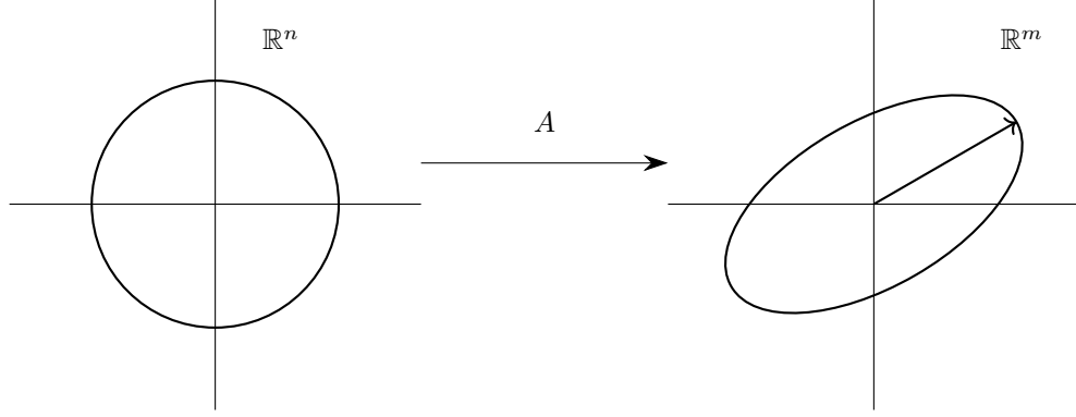
Figure 11: The norm of A is the length of the major axis of the ellipsoid. Given that \dim X = n , imagine the n -dimensional unit ball in X being transformed under A . The image of the ball should be an ellipsoid (of dimension \leq m ) in U .
