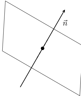
Figure 10: The linear operator that rotates around a vector v by an angle \theta has an eigendecomposition of the span of v as shown (with eigenvalue 1) and the 2-dimensional plane (having two complex eigenvalues).
