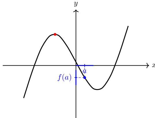
Figure 9: A cubic can fail to be locally invertible at a turning point, but behave regularly at nearby non-turning points.
