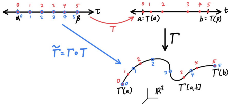
Figure 40: Note that the points are labeled 0, 1, 2, 3, 4, 5 do not represent numerical values, but rather the order in which the points are parameterized. We can see from this ordering that T is monotonic.
