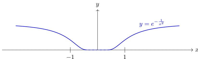
Figure 42: Graph of the function y = e^{-1/x^2} . This function equals 0 at x = 0 and approaches 1 as |x| approaches infinity. One can verify that the derivative f^{(k)}(0) = 0 for all k and hence the Taylor series is identically equal to 0, while f(x) \neq 0 if x \neq 0 .
