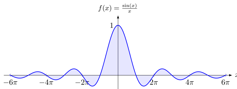
Figure 38: Plot of the function f(x) = \frac{\sin(x)}{x} . The integral is improper due to the unbounded domain (-\infty, +\infty) , despite the function itself being bounded.
