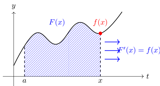
Figure 35: This theorem amazingly tells us that the rate at which the integral F is increasing at x (represented by the increasing area under the curve of f ) is equal to the value of f at the point x itself!
