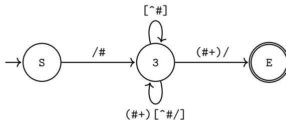
Figure 21: The NFA after eliminating state 4. The paths through state 4 are converted into a direct edge to E and an additional loop component on state 3.
