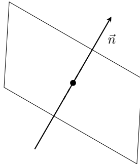
Figure 15: The linear operator that rotates around a vector v by an angle \theta has an eigendecomposition of the span of v as shown (with eigenvalue 1) and the 2-dimensional plane (having two complex eigenvalues).
