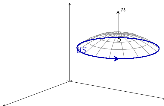
Figure 28: The orientation unit vector n of S induces the positive orientation of \partial S , denoted \partial S^+ . Visually, if you are walking along the curve with your head is pointing in the same direction as the unit normal vectors while the surface is on the left then you are walking in the positive direction on \partial S .
