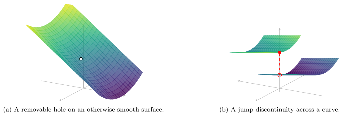
Figure 19: Two typical discontinuities that can still occur in integrable functions: a removable hole and a jump discontinuity.
