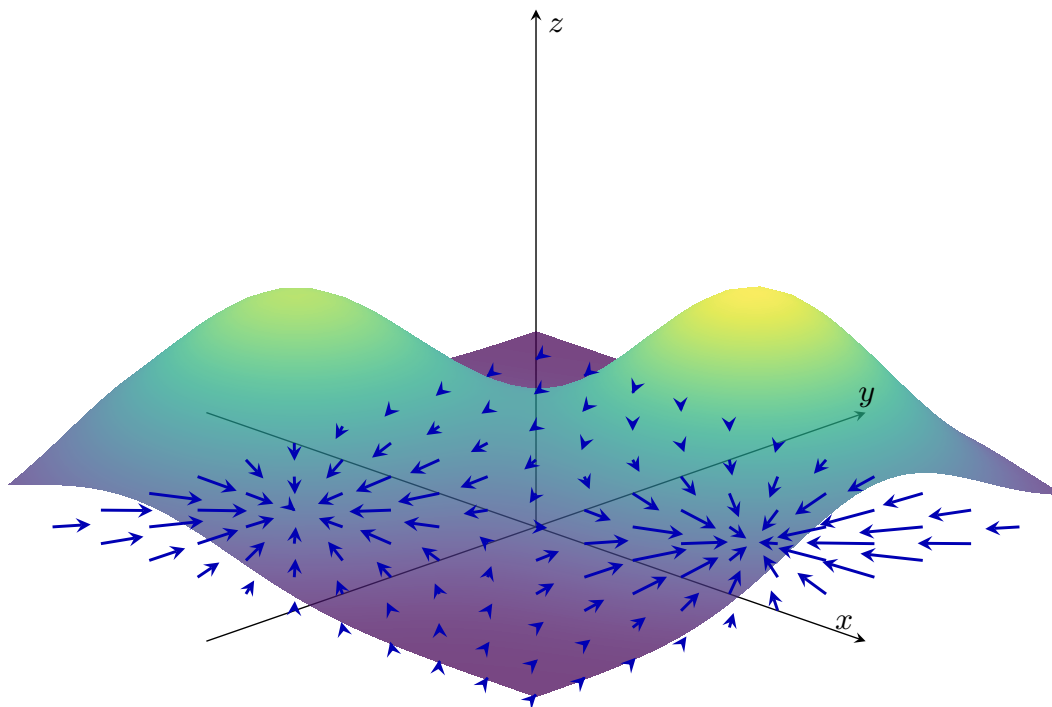
Figure 26: The vector field on the xy -plane is a conservative vector field since it is the gradient of the scalar field f(x, y) = 2.2e^{-((x-1.2)^2+(y-0.8)^2)/1.6} + 1.9e^{-((x+1.3)^2+(y+0.9)^2)/1.8} + 0.12 . The arrows on the xy -plane point in the direction of steepest ascent on the surface.
