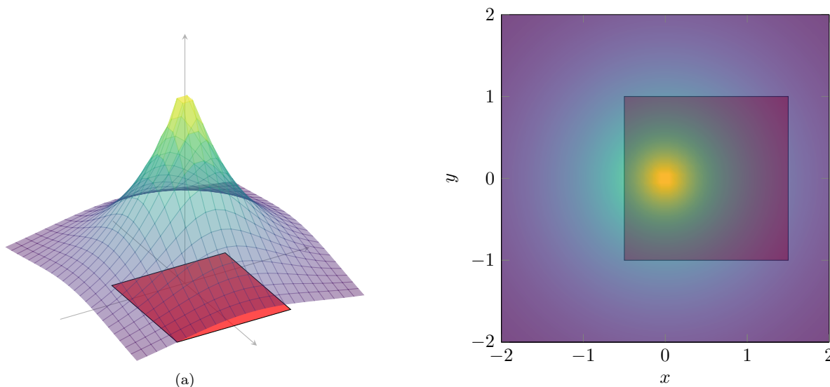
Figure 18: Two interpretations of double integral \iint_B e^{-\sqrt{x^2+y^2}} dx dy . On the left, we can view it as the area under a surface. On the right, we view it as the mass of a 2-dimensional sheet lying on [-0.5, 1.5] \times [-1, 1] of varying density defined by function f(x, y) .
