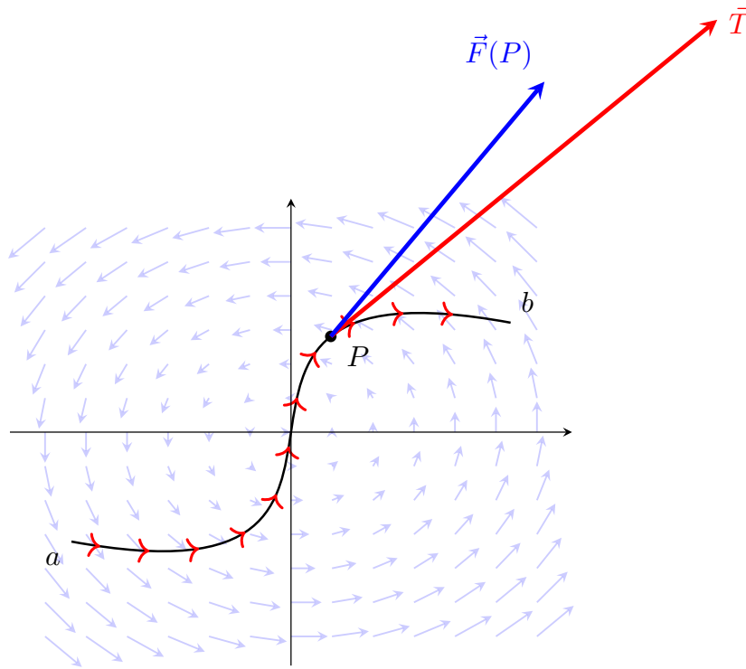
Figure 24: Visualizing a path integral. At a specific point P along the oriented curve, the red tangent vector \vec{T} points along the path, while the solid blue vector \vec{F}(P) represents the local vector field at that exact location. The path integral \int_C \vec{F} \cdot d\vec{r} accumulates the dot product of these two vectors at every point along the curve.
