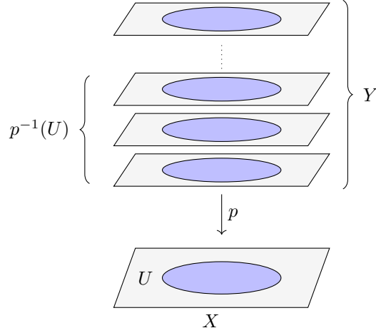
Figure 5: The best way to visualize this is to think of a “stack of pancakes.” Consider Y = X \times \mathbb{Z} and let p(x, z) = x be a projection. Given some open U \subset X , p^{-1}(U) = U \times \mathbb{Z} , with each slice V_z = U \times \{z\} mapping homeomorphically onto U .
