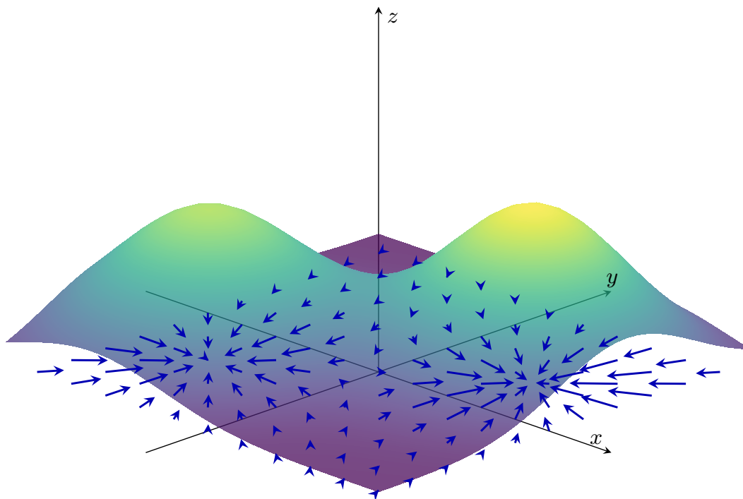
Figure 22: The vector field on the xy -plane is a conservative vector field since it is the gradient of the scalar field f(x, y) = 2.2e^{-((x-1.2)^2+(y-0.8)^2)/1.6} + 1.9e^{-((x+1.3)^2+(y+0.9)^2)/1.8} + 0.12 . The arrows on the xy -plane point in the direction of steepest ascent on the surface.
