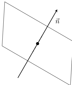
Figure 13: The linear operator that rotates around a vector v by an angle \theta has an eigendecomposition of the span of v as shown (with eigenvalue 1) and the 2-dimensional plane (having two complex eigenvalues).
