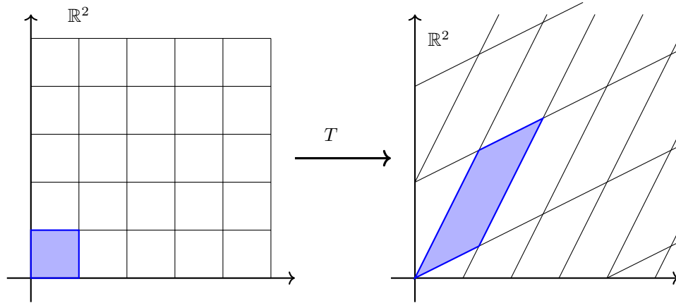
Figure 10: An important way to visualize determinants is by using the linear map visualization introduced before. That is, the determinant is the area of the transformed shaded unit square.
