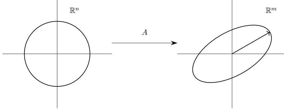
Figure 14: The norm of A is the length of the major axis of the ellipsoid. Given that \dim X = n , imagine the n -dimensional unit ball in X being transformed under A . The image of the ball should be an ellipsoid (of dimension \leq m ) in U .
