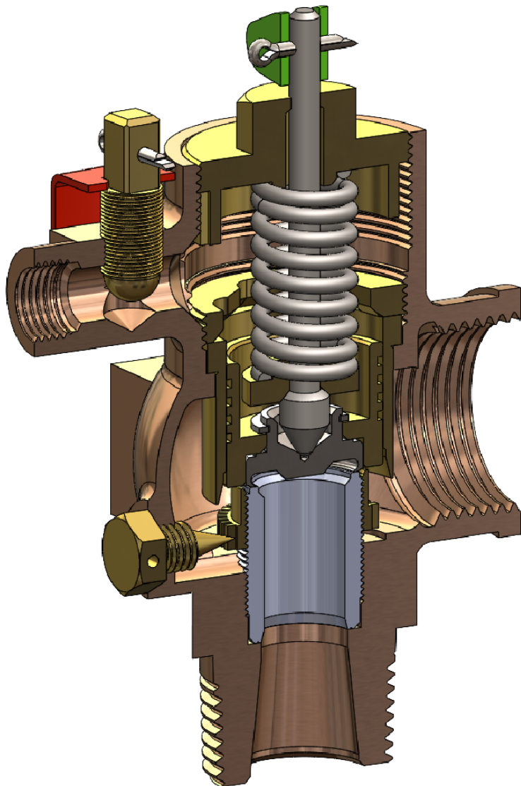
SP-1 Structure
